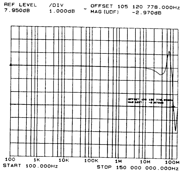
Figure 7 - Frequency Response
