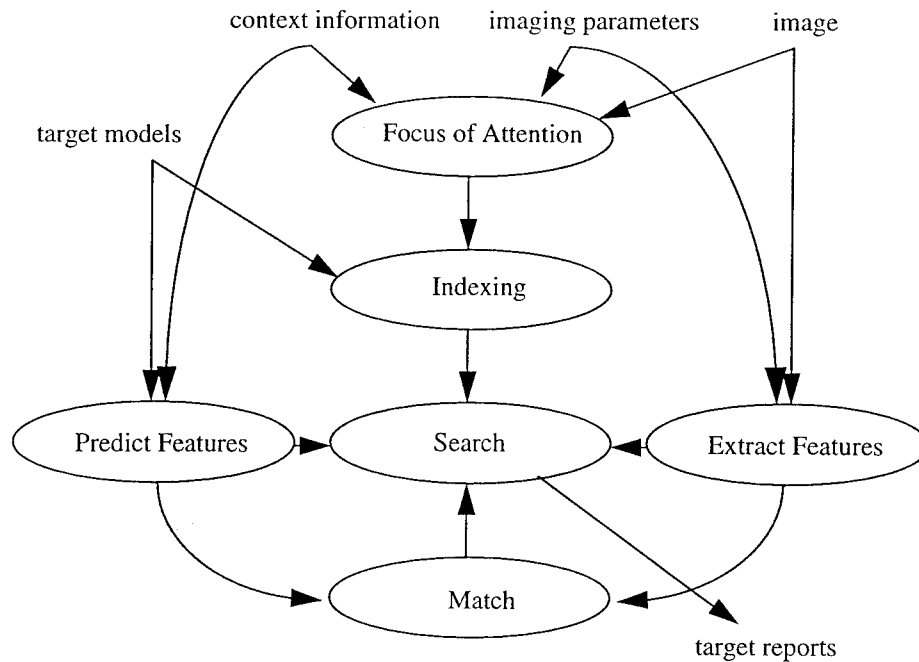
FIGURE 1. An architecture for model-driven ATR, after [45].
