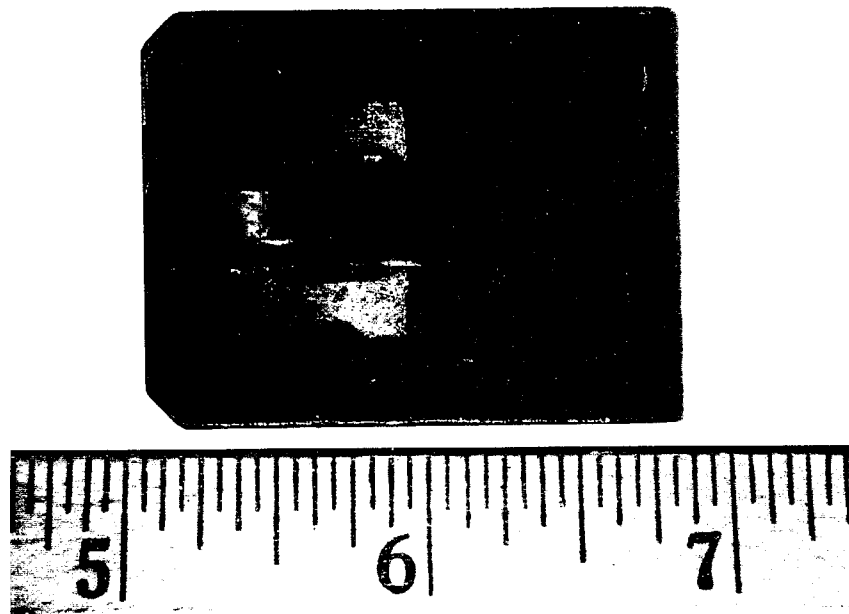
FIGURE 10 Top view of the individual locking block showing excessive machine marks. Surface finish was determined to be out of specification. Mag. 1.5x.
