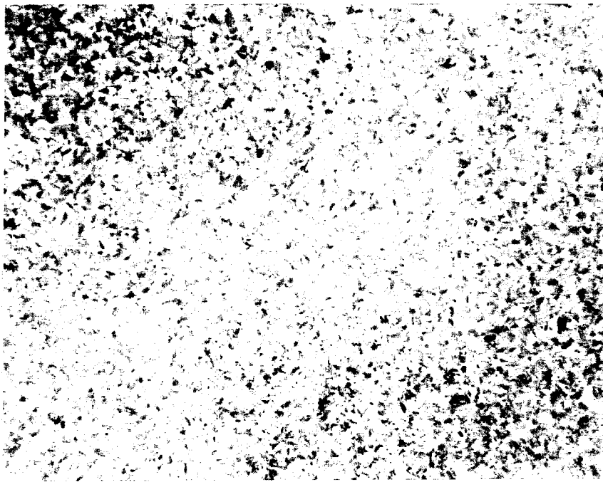
FIGURE 39 Spiral spring ("Top") microstructure consisting of a fine tempered martensite consistent with the required heat treatment. Fry's reagent. Mag. 500x
