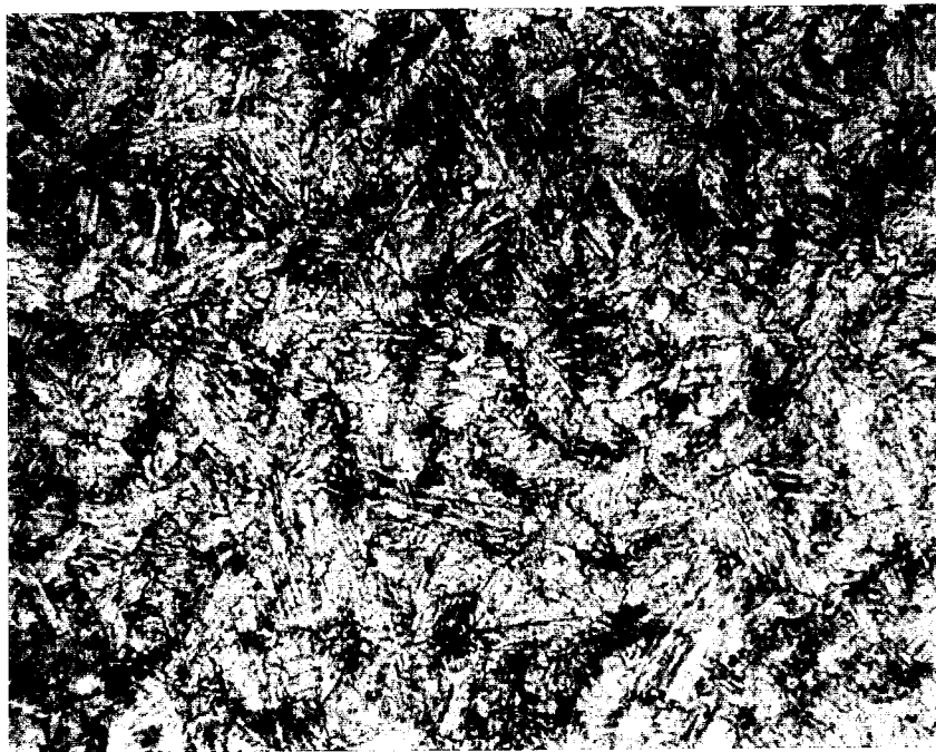
FIGURE 23 Firing pin microstructure (Maraging, Grade 300) consisting of low carbon martensite, consistent with prior heat treatment. Fry's reagent. Mag. 300x.
