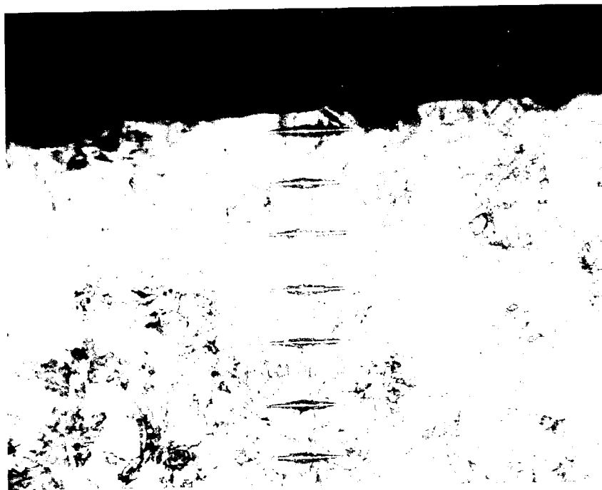
FIGURE 29 Microhardness profile conducted to verify nitrided case on the "After-Market" bolt shaft, bottom. No significant hardness gradient was noted. Fry's reagent. Mag. 300x.
