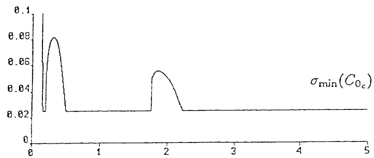
Figure 4.3: \sigma_{\min}(C_0(t)) and \sigma_{\min}(C_{0_c}(t))
