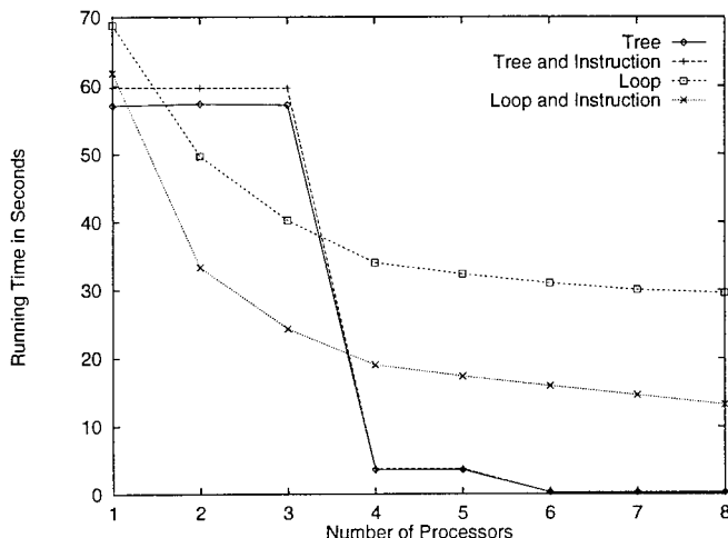
Figure 3.1: Comparison of Four Parallelizations, Varying Processors
