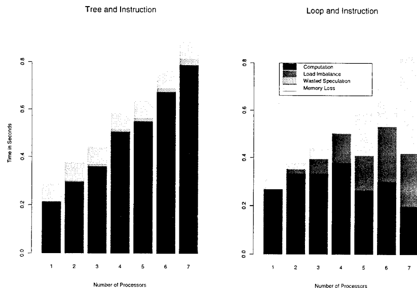
Figure 4.7: Predicate Profiles of Two Parallelizations on SGI; Many Solutions, Dense Input
