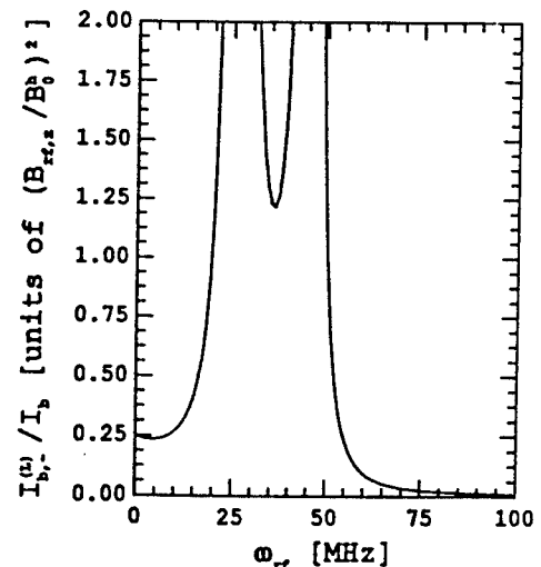
FIG. 5. Relative first-order sideband intensity I_{b,-}^{(L)}/I_b for a static magnetic field B_0^h and a linearly polarized field of amplitude B_{\text{rf},x} for ^{57}\text{Fe} nuclei in iron. The relative intensity I_{b,-}^{(L)}/I_b has resonances at \omega_{\text{rf}}=\omega_e , \omega_{\text{rf}}=\omega_g . The direction of observation is perpendicular to the plane of the applied field. The \gamma -ray intensities are averaged over the polarization.
