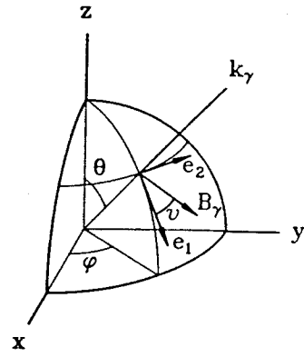
FIG. 1. Orientation of the magnetic field B_\gamma and of the wave vector k_\gamma of a quantum of \gamma radiation emitted by a ^{57}\text{Fe} nucleus.
