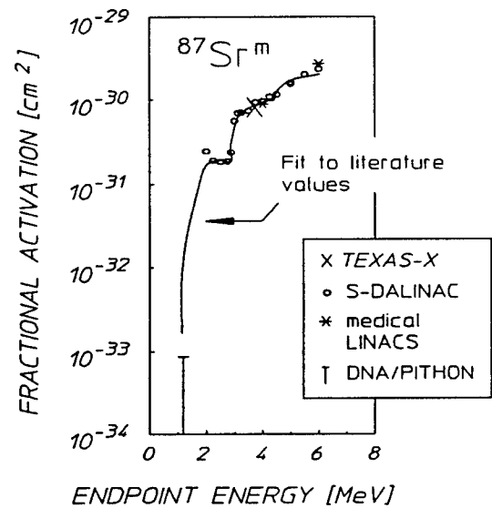
Figure 2: Excitation function showing measured fractional activation, A_f for the reaction ^{87}\text{Sr}(\gamma, \gamma)^{87}\text{Sr}^m as a function of bremsstrahlung endpoint, E_0 . The solid curve plots values computed from Eq. (3) using gateway parameters found in the literature and calculated photon spectra.
