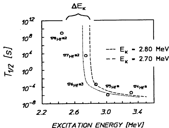
Figure 7: Halflife as a function of excitation energy for the four- and five-quasiparticle Hf isomers of Fig. 6. The curves represent calculated dipole-transition halflives for the deexcitation of the isomers for different choices for the gateway energy and further bound the possible positions of such a level.
