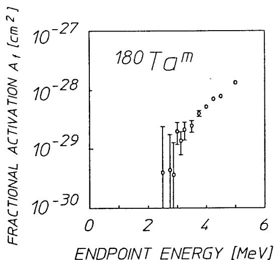
Figure 3: Excitation function showing fractional activation, A_f for the reaction ^{180}\text{Ta}^m(\gamma,\gamma)^{180}\text{Ta} as a function of bremsstrahlung endpoint, E_0 . These data demonstrate the dumping of an isomeric population to freely-radiating states with trigger x rays.
