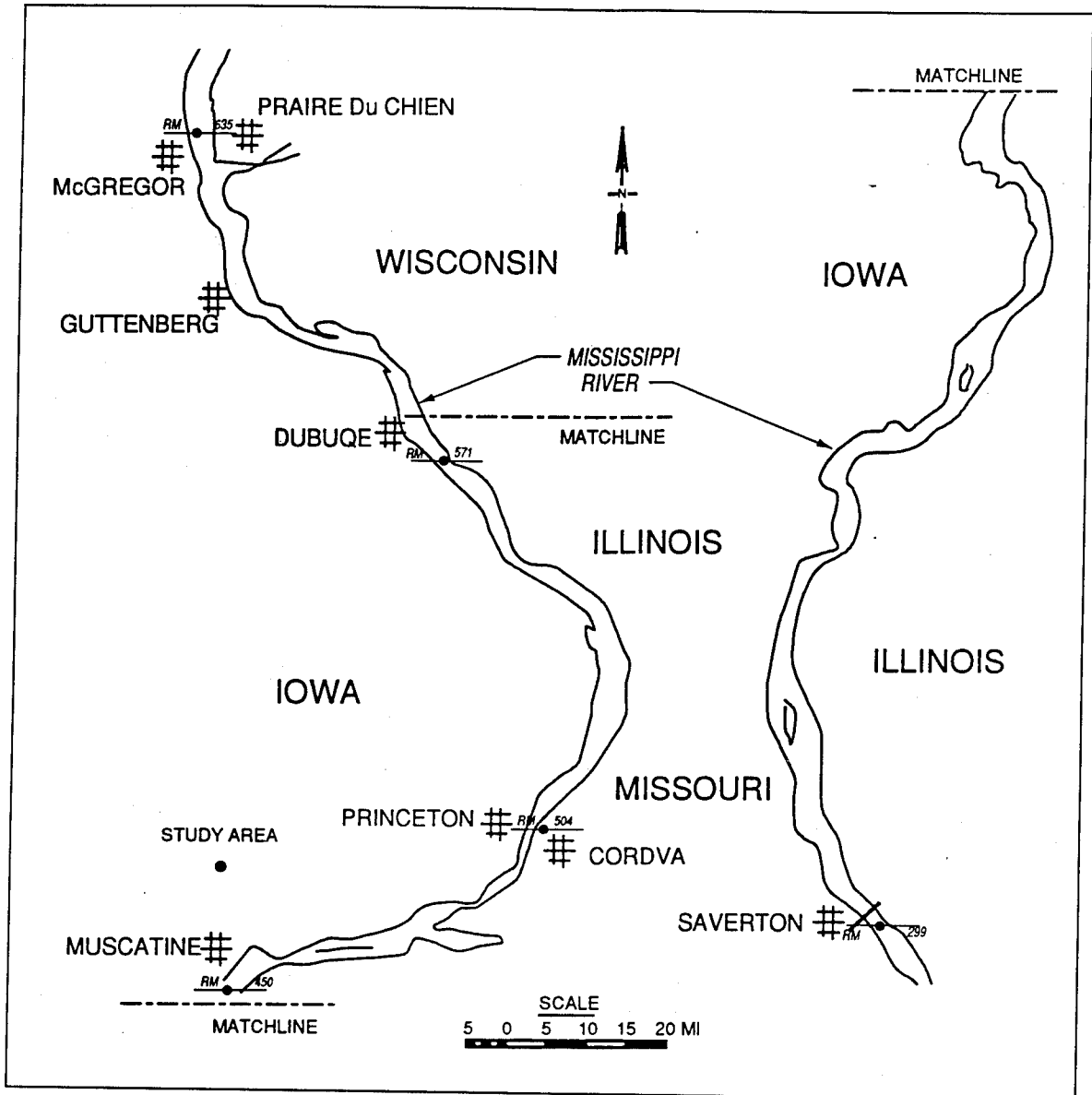
Figure 1. Location of five mussel beds chosen for detailed study in UMR, 1989-1994
