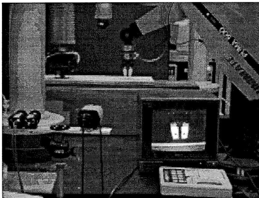
Figure 18: Laboratory setup used for performing vision/force servoing experiments.
