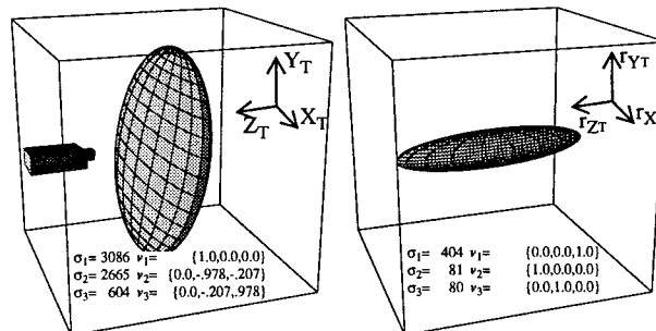
Figure 7: Resolvability Ellipsoids: monocular system, f=12\text{mm} , depth=0.5m, 2 features located in the task frame at (0.1m,0.1m,0) and (-0.1m,0.1m,0).
