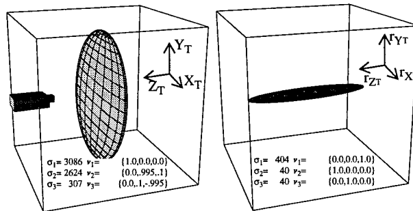
Figure 6: Resolvability Ellipsoids: monocular system, f=24\text{mm} , depth=1.0m, 2 features located in the task frame at (0.1m,0.1m,0) and (-0.1m,0.1m,0).
