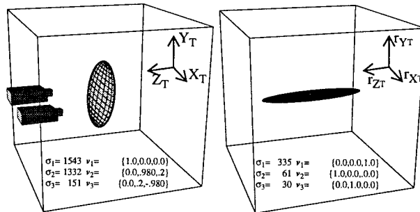
Figure 10: Resolvability Ellipsoids: stereo pair-parallel optical axes, f=12\text{mm} , b=20\text{cm} , depth= 1.0\text{m} , 1 feature located in the task frame at (0,0.2m,0).
