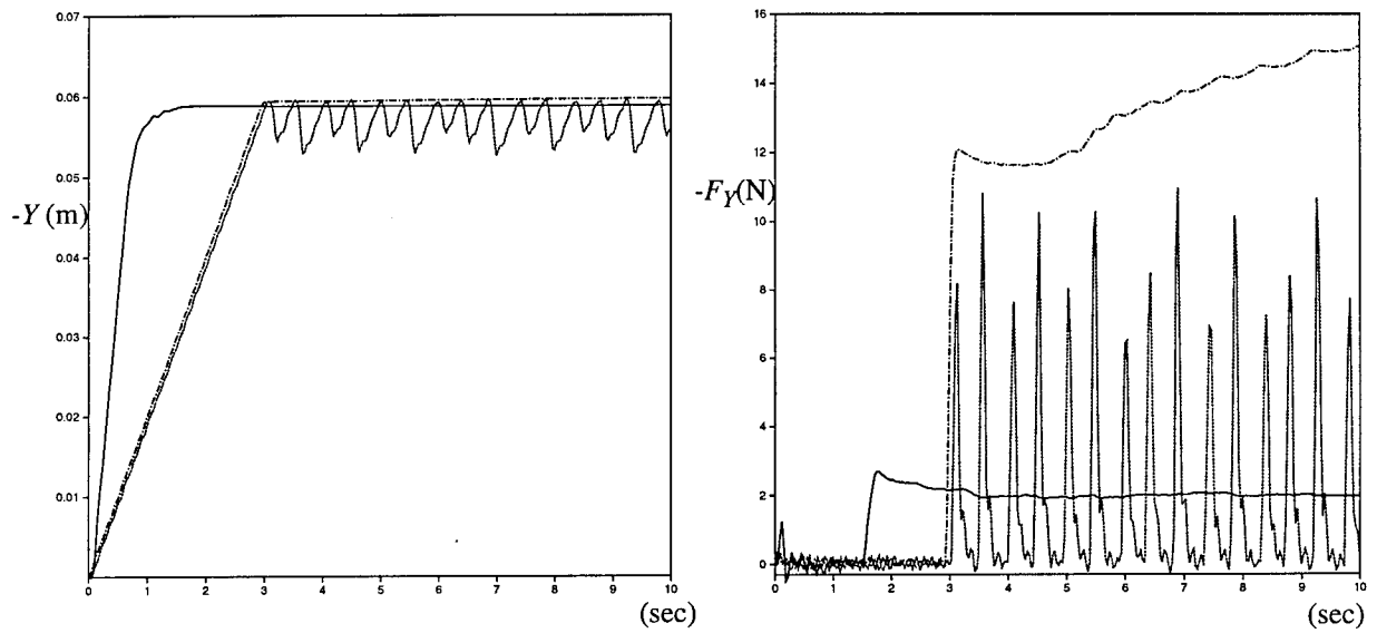
Figure 27: Combined plots of vertical position and measured force during impact for force/vision control, damping force control, and a guarded move.
