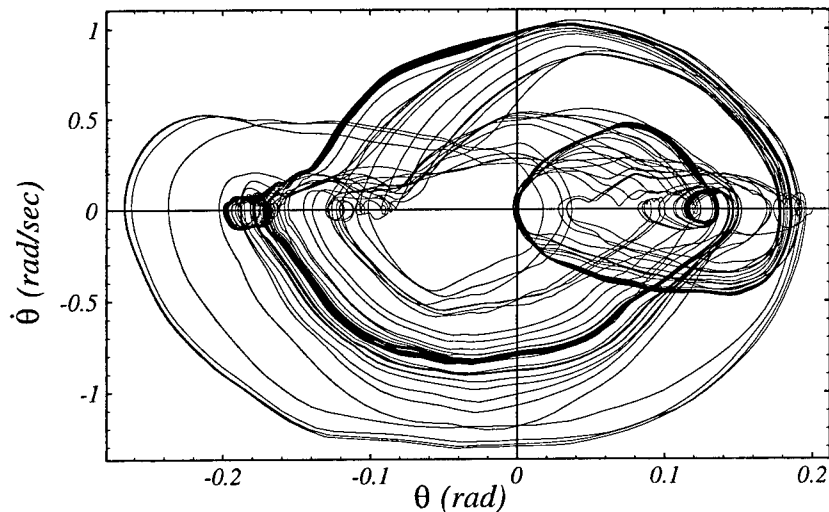
Figure 28: The pendulum trajectory appears to form a possibly chaotic attractor in phase space.
