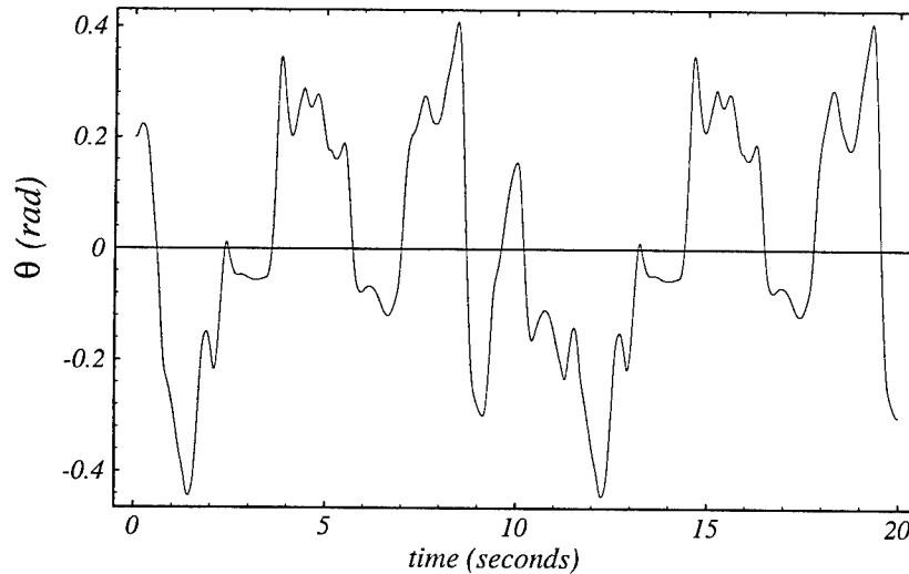
Figure 31: The neural network forms a stable controller.
