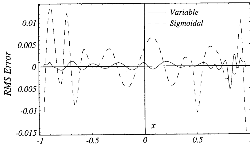
Figure 4: RMS approximation error for the median variable network and the median sigmoidal network.
