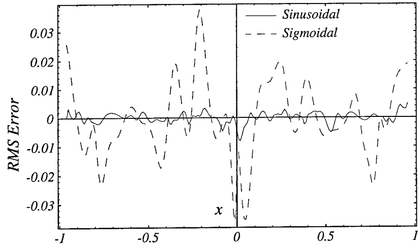
Figure 15: RMS approximation error for the median sinusoidal network and the median sigmoidal network.
