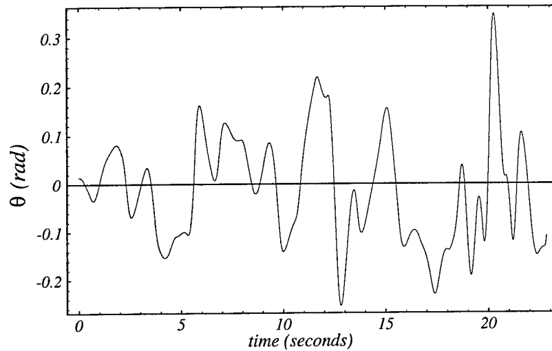
Figure 24: Pendulum angle for the complete successful training run of 23 seconds.
