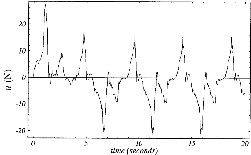
Figure 27: Control output generated by the neural network controller.
