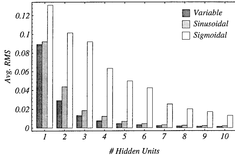
Figure 11: The RMS error decreases much faster in the variable and sinusoidal networks than in the sigmoidal network.
