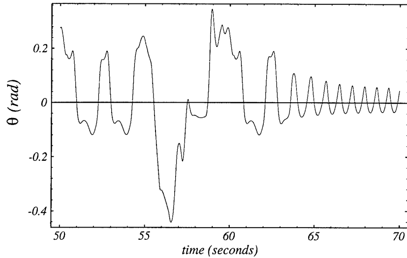
Figure 33: The neural network controller converges to encircle the origin in phase space.
