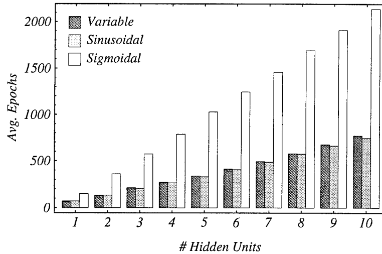
Figure 17: Learning is again much faster in the variable and sinusoidal networks than the sigmoidal network.
