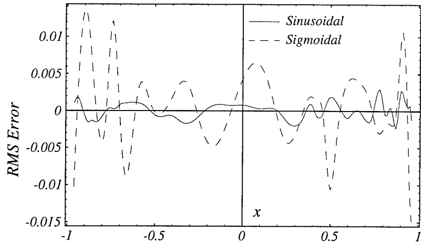
Figure 5: RMS approximation error for the median sinusoidal network and the median sigmoidal network.
