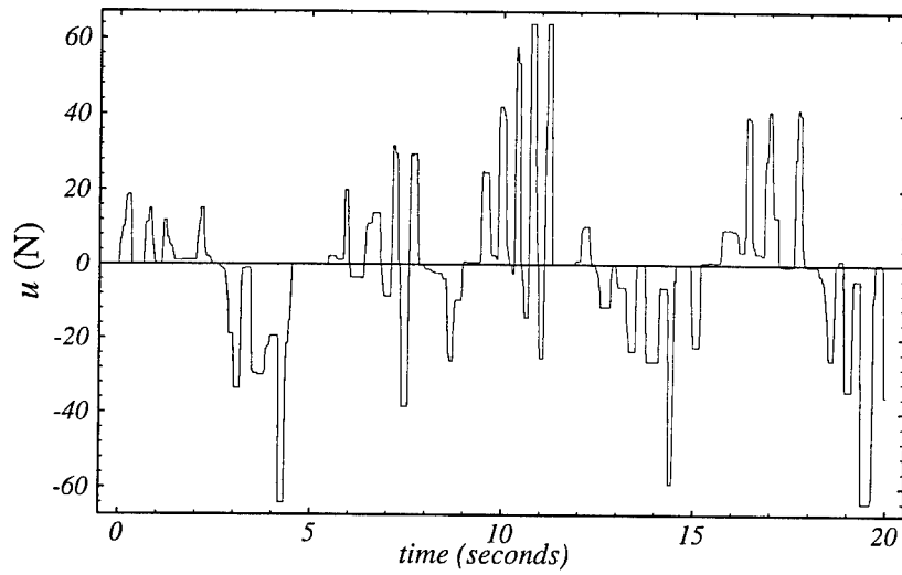
Figure 30: Control forces for the second human controller are higher than for the first case.
