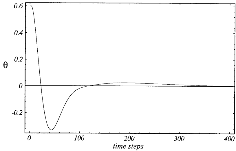
Figure 20: The initial pendulum angle starts outside the range of the training data for the network.
