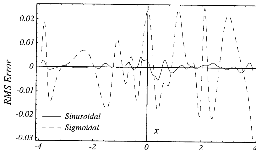
Figure 10: RMS approximation error for the median sinusoidal network and the median sigmoidal network.
