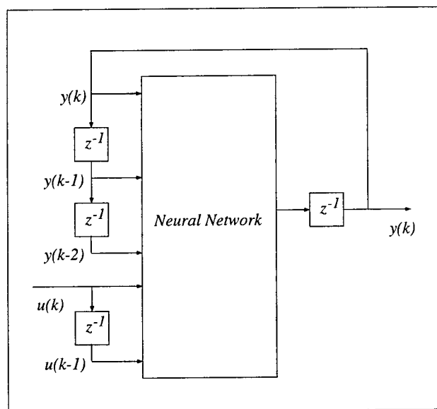
Figure 18: A dynamic system can be mapped onto a static feedforward neural network.
