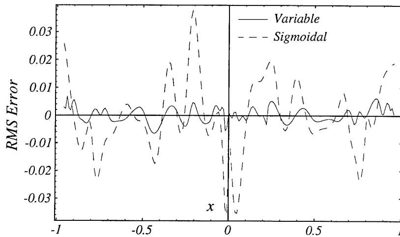
Figure 14: RMS approximation error for the median variable network and the median sigmoidal network.
