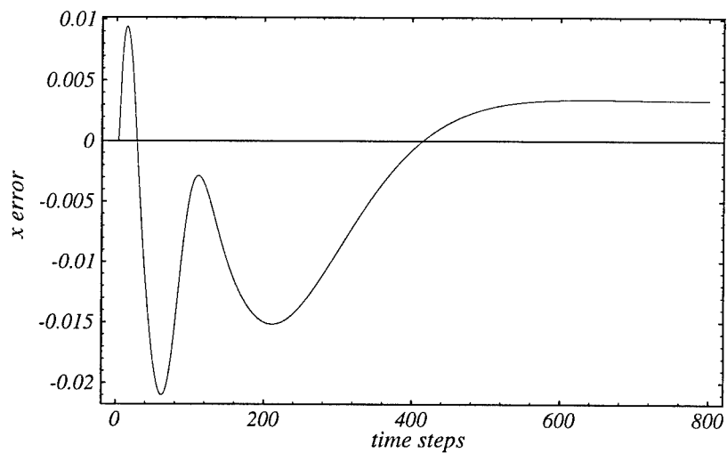
Figure 21: The neural network controller exhibits a small steady state error of approximately 3 mm.
