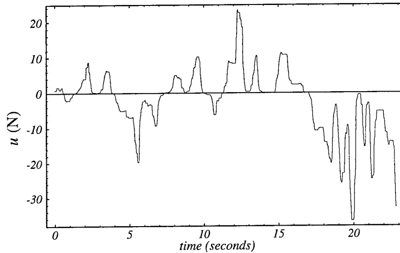
Figure 25: Control force for the complete successful training run of 23 seconds.
