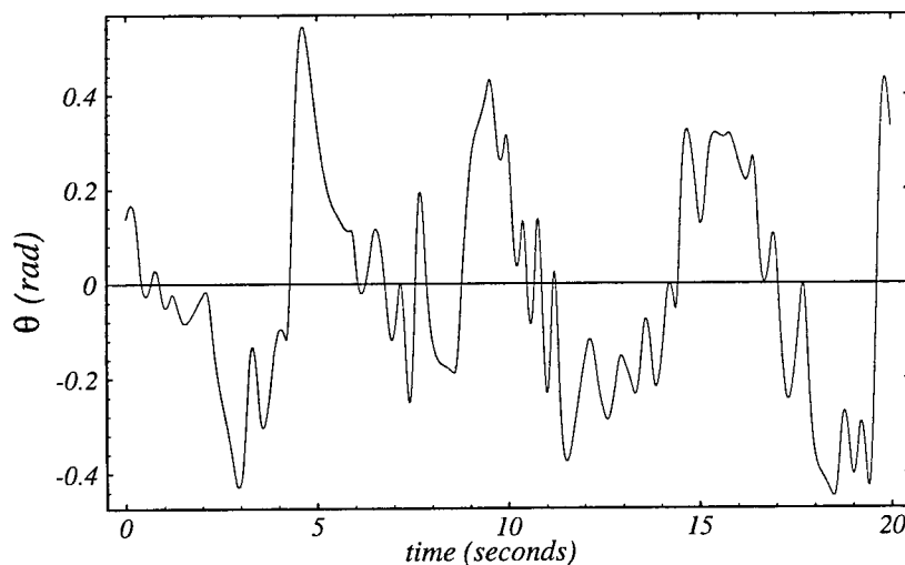
Figure 29: Part of the 60 second successful run for the second human controller.
