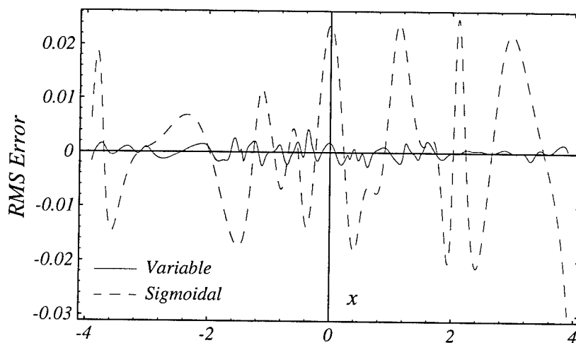
Figure 9: RMS approximation error for the median variable network and the median sigmoidal network.
