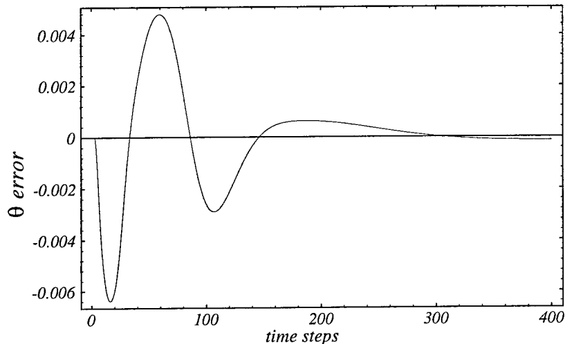
Figure 22: The pendulum angle converges to zero steady state error.
