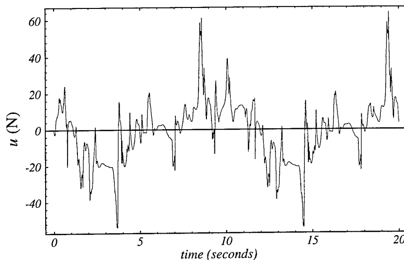
Figure 32: The neural network controller converges to encircle the origin in phase space.
