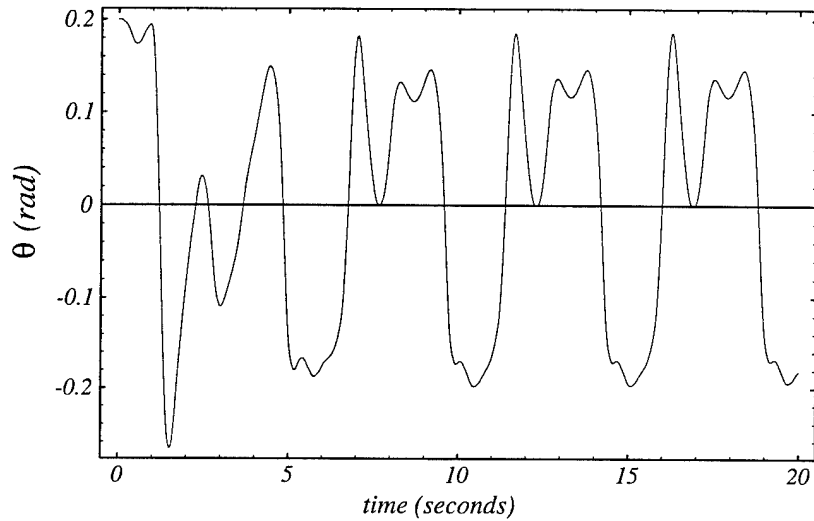
Figure 26: The neural network forms a stable, but nonconvergent controller.
