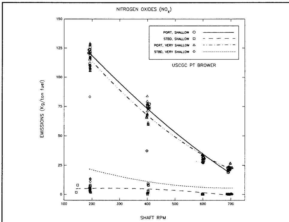
Figure 7 PT BROWER NO x (kg/tonne fuel) versus Engine Speed
