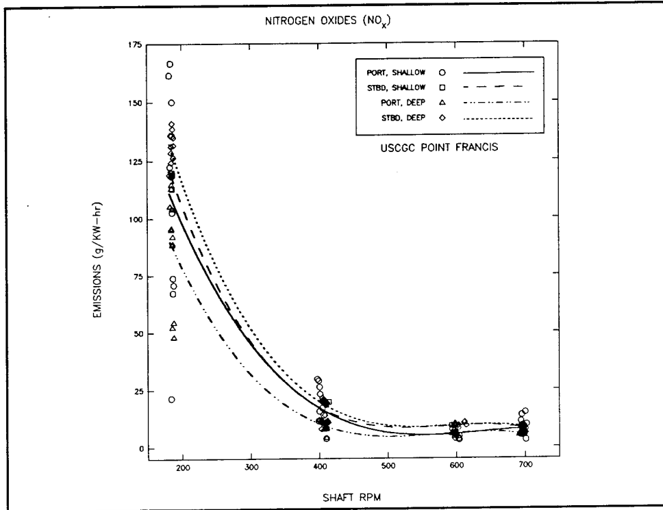
Figure 1 PT FRANCIS NO x (g/kw-hr) versus Engine Speed
