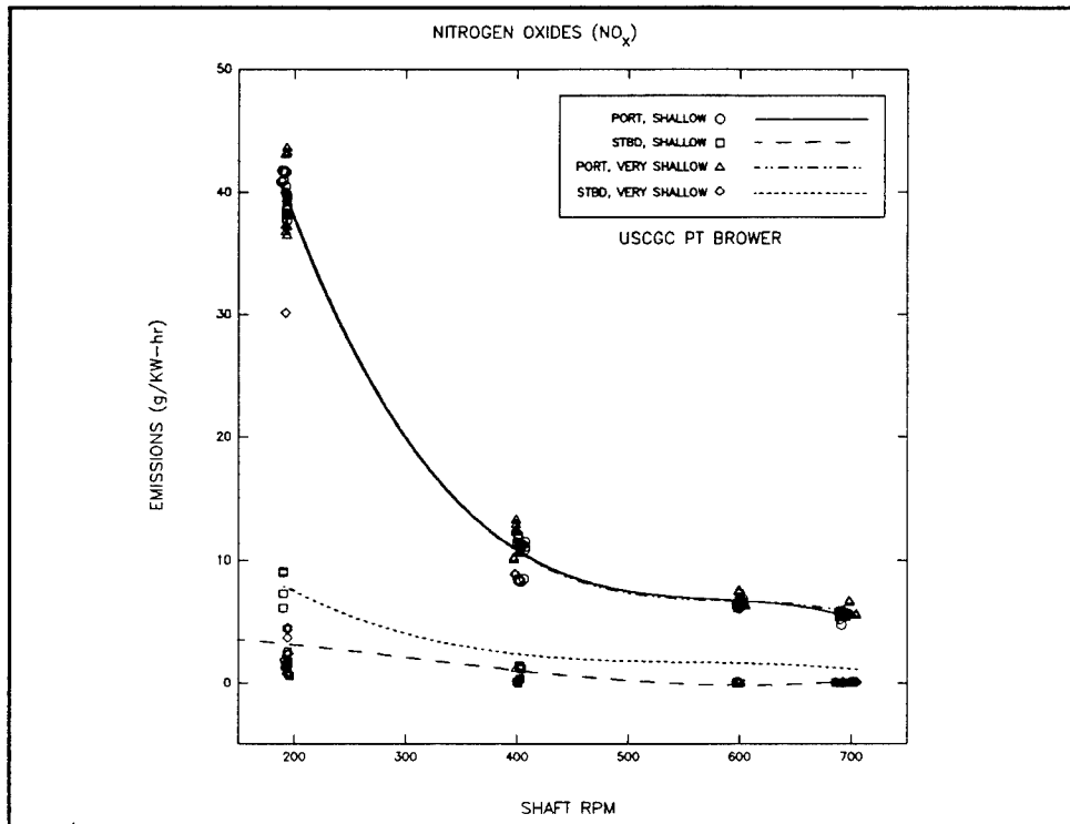
Figure 6 PT BROWER NO x (g/kw-hr) versus Engine Speed
