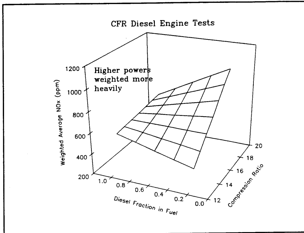
Figure 20 CFR Engine Higher Powers
