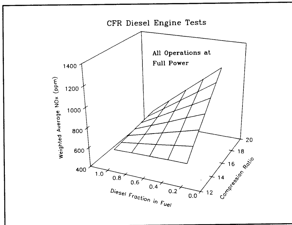
Figure 19 CFR Engine Full Power
