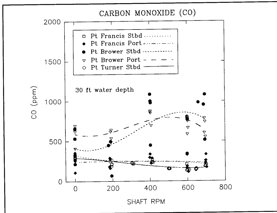
Figure 18 Combined CO Results (Raw Data)
