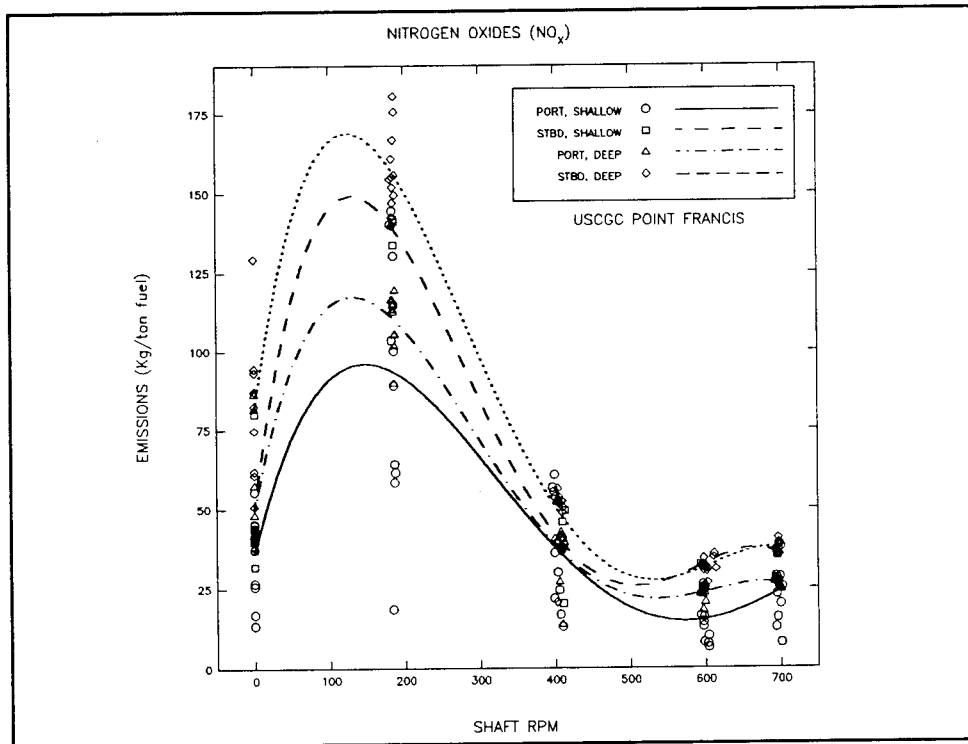
Figure 2 PT FRANCIS NO x (kg/tonne fuel) versus Engine Speed
