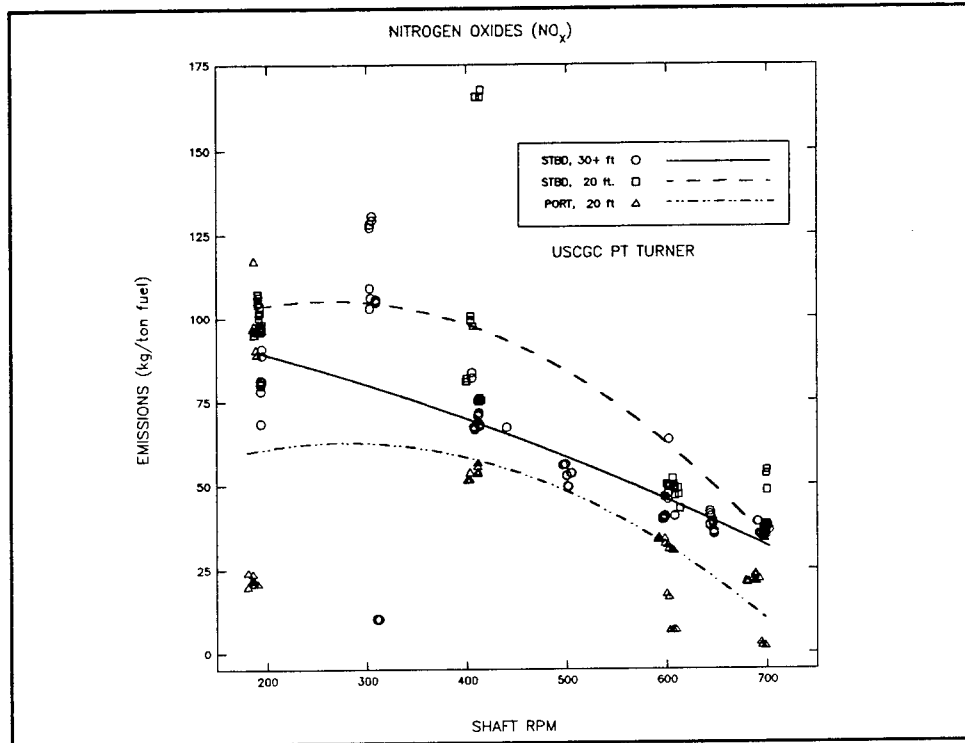
Figure 14 PT TURNER NO x (kg/tonne fuel) versus Engine Speed
