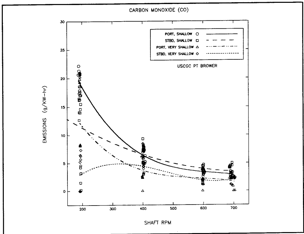
Figure 8 PT BROWER CO (g/kw-hr) versus Engine Speed
