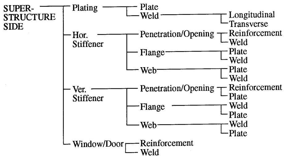
Figure B.3: SID - Super-Structure Side Components
