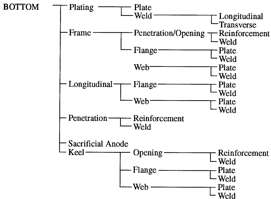
Figure B.2: SID - Bottom Components
