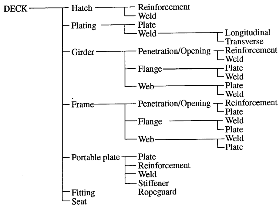
Figure B.4: SID - Deck Components
