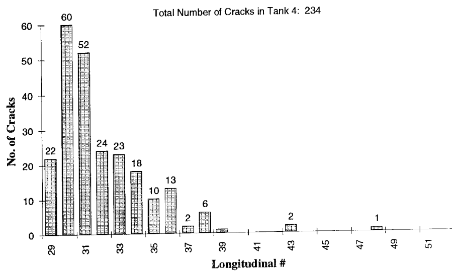
Figure 3.14: Side Shell Longitudinal Cracks in Tank 4
