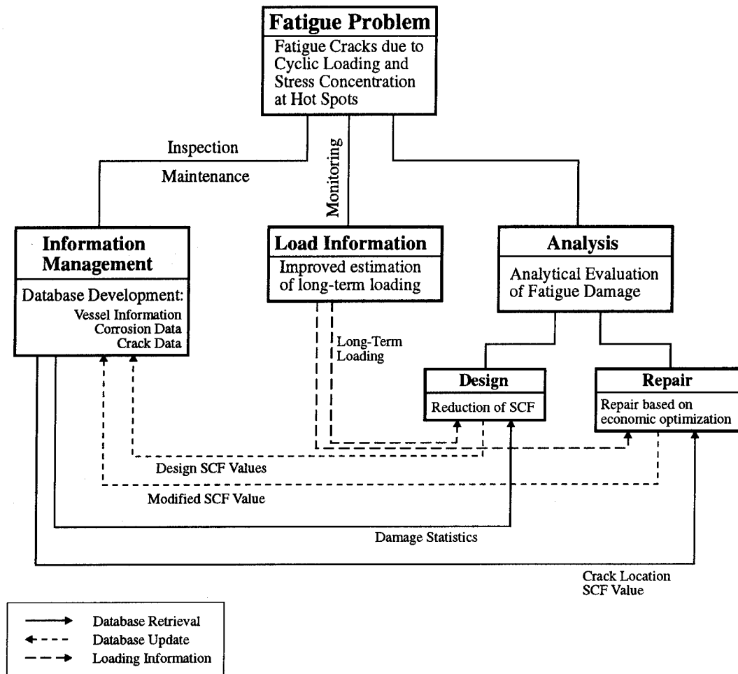
Figure 2.1: Schematic View of the Fatigue Problem
