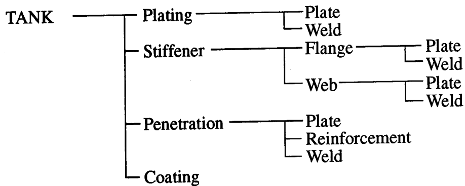
Figure B.9: SID - Tank Components
