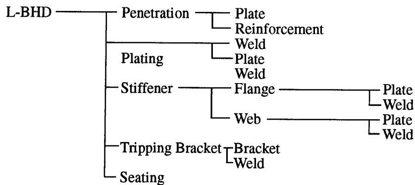
Figure B.5: SID - Longitudinal Bulkhead Components
