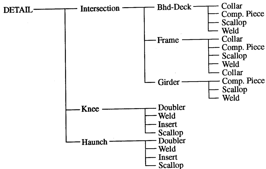
Figure B.11: SID - Detail Components
