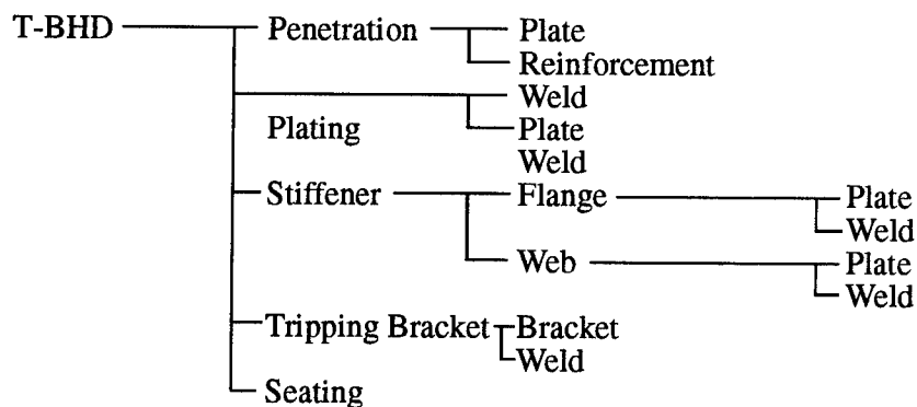
Figure B.6: SID - Transverse Bulkhead Components
