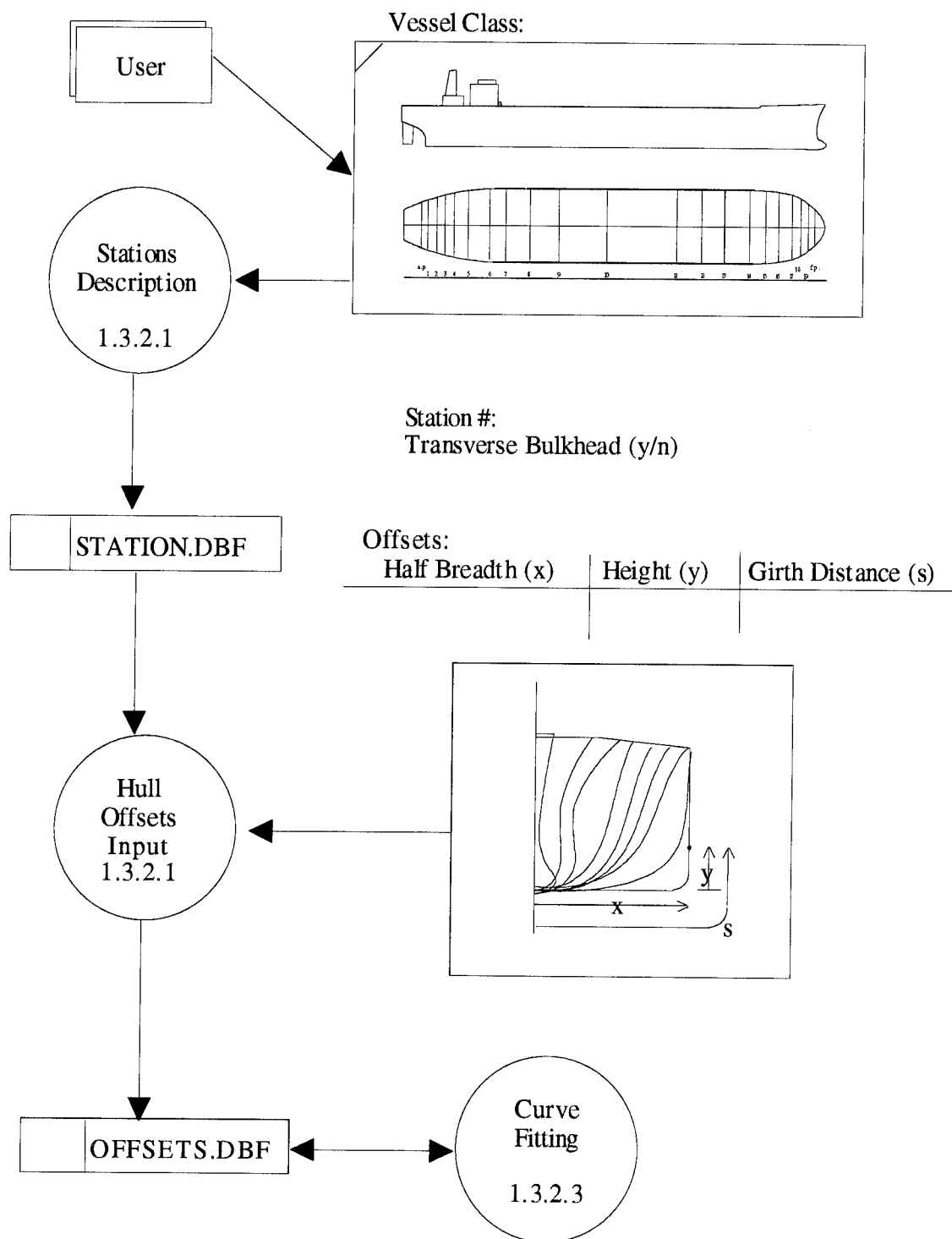
Figure 3.18: DCL - Hull Geometry Description
