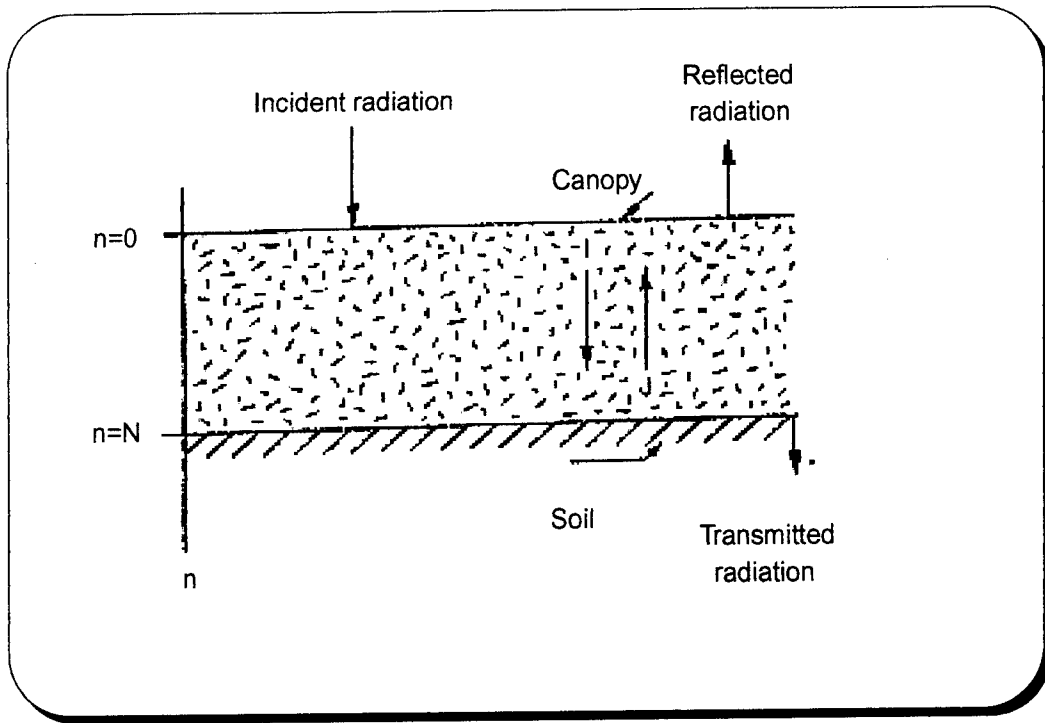
Figure 5. Geometry of a plant canopy. (Allen, 1969)
