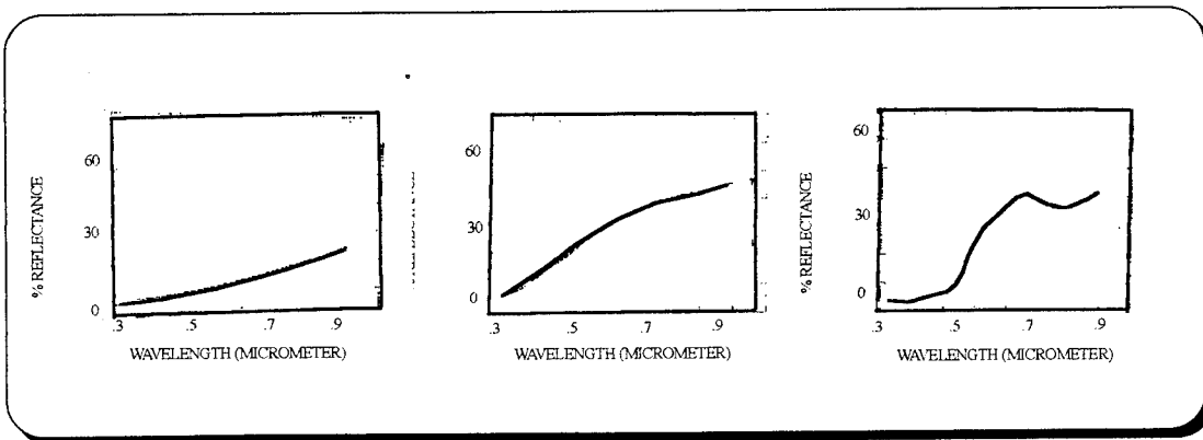
Figure 8. Characteristic spectra of Type I, Type II, and Type III soils. (Condit, 1970)
