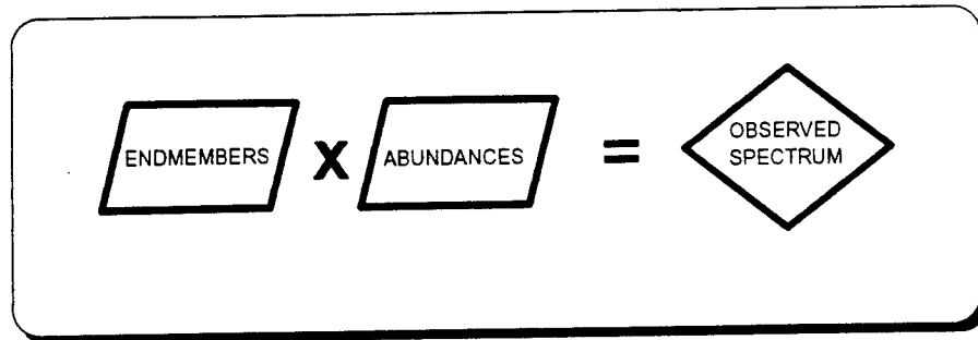
Figure 13. Linear spectral mixing. (Boardman, 1990)
