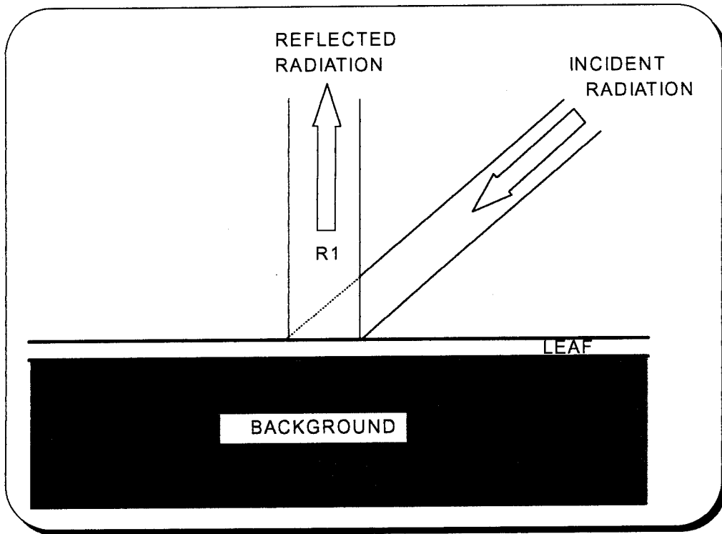
Figure 9. Single leaf on a plane background (Lillesaeter, 1982)
