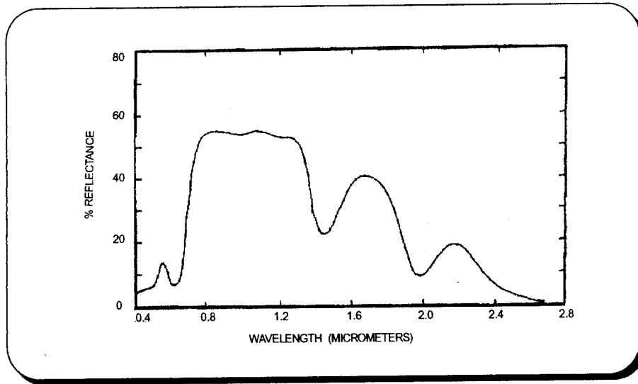
Figure 1. Typical spectrum of a green leaf. (Knipling, 1970)
