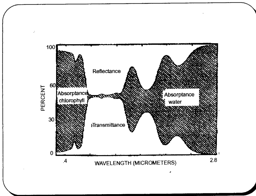
Figure 2. Reflectance, absorptance, and transmittance spectra of a plant leaf. (Knipling, 1970)
