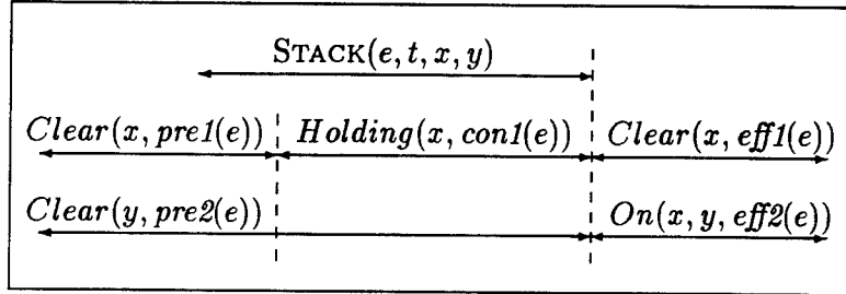
Figure 2.5: Necessary conditions for stacking x on y
