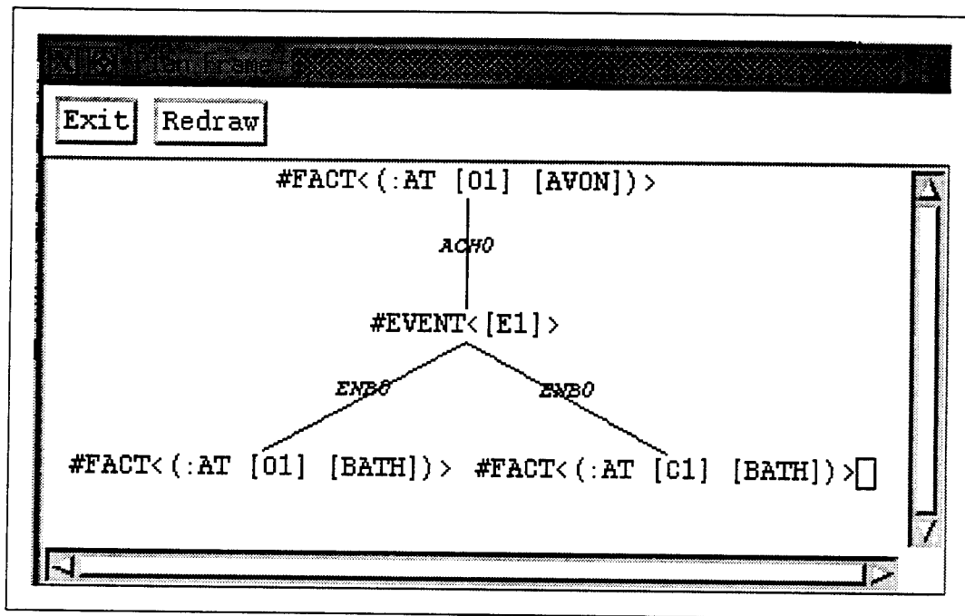
Figure 4.4: Sample plan graph: CLIM display
