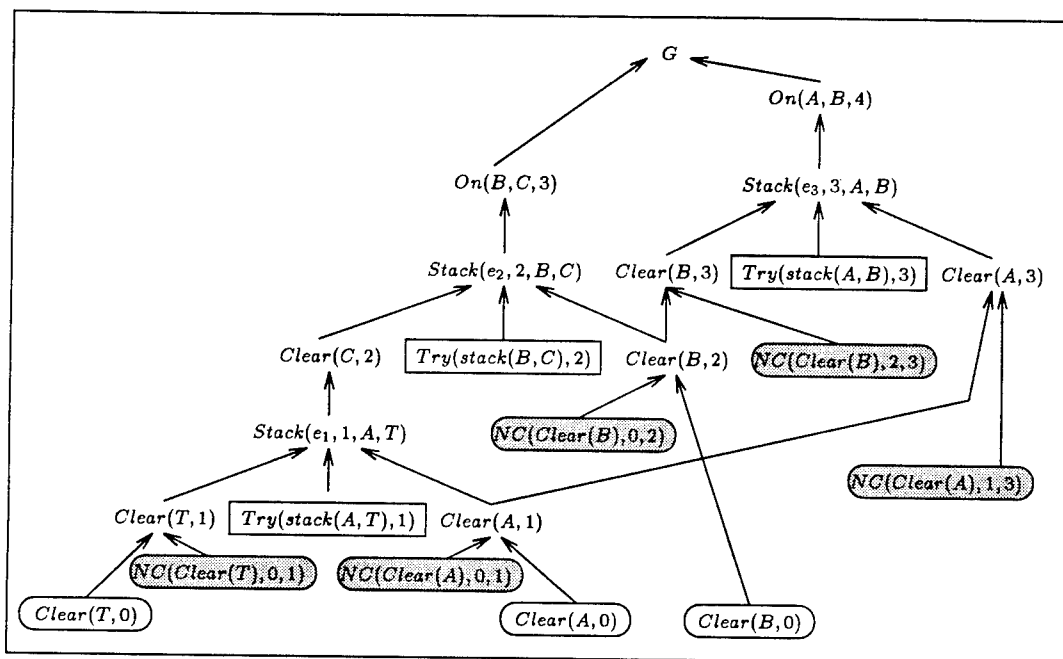
Figure 3.9: A supported plan for the Sussman problem
