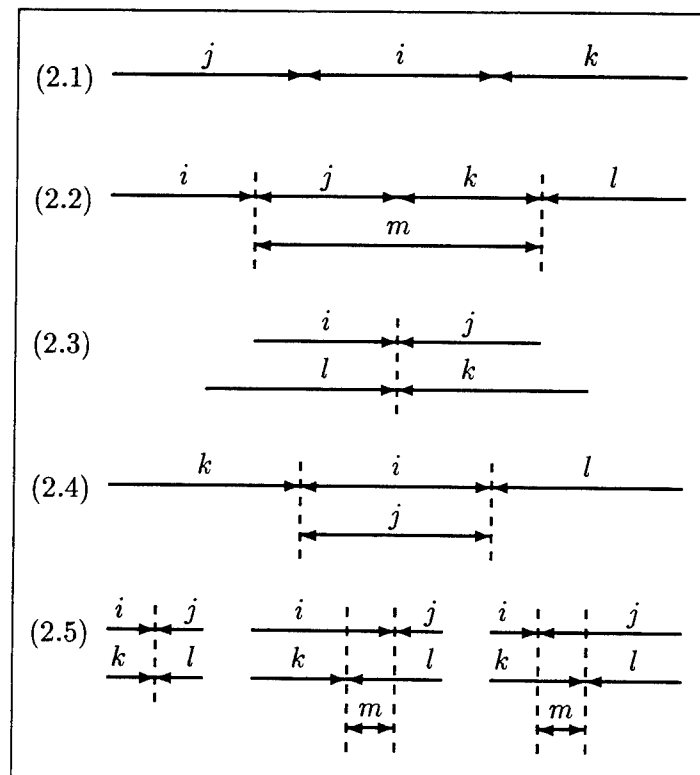
Figure 2.3: The axiomatization of time periods
