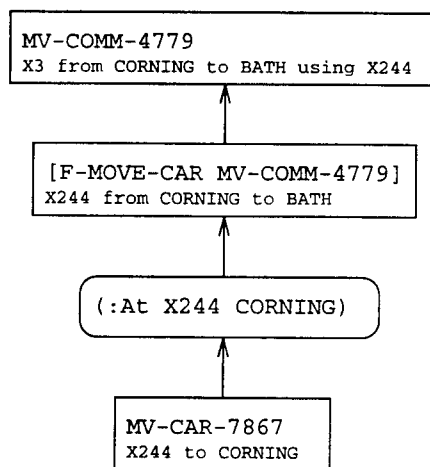
Figure 4.12: Plan graph after incorporating moving a boxcar to Corning
