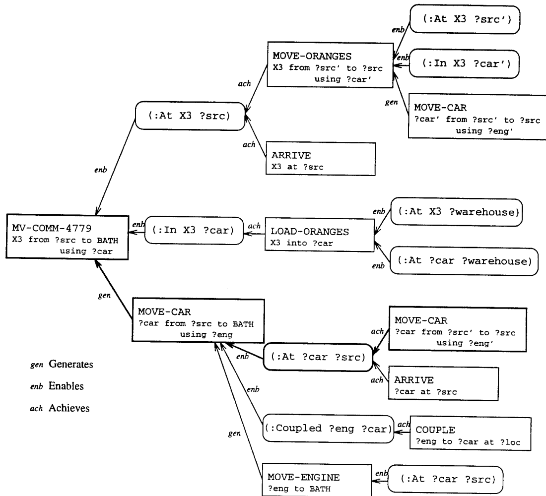
Figure 4.11: Expansion of plan graph during incorporation
