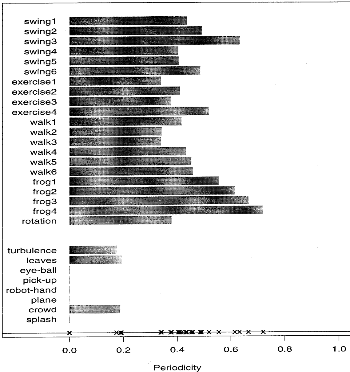
Figure 1: Periodicity measure for Periodic and Nonperiodic sequences
