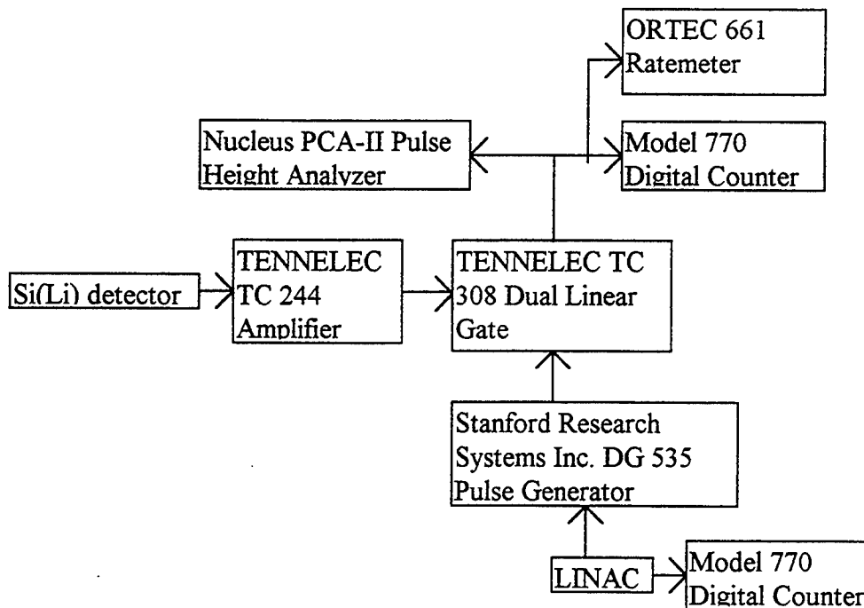
Figure 5. Electronics setup.
