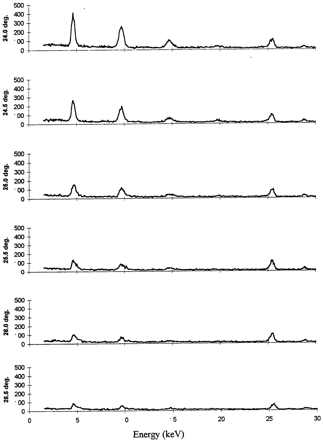
Figure 12. Raw 2.5° Mosaicity Spectra at E_c = 97.62 MeV(Cont.).
