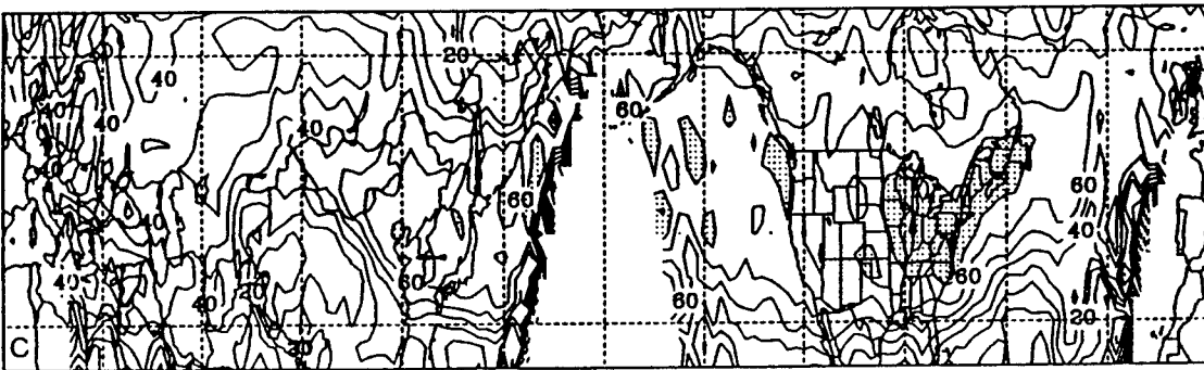
Figure 18. As in Fig. 14 except for channel 3 MSU and 500-mb vorticity correlations.
