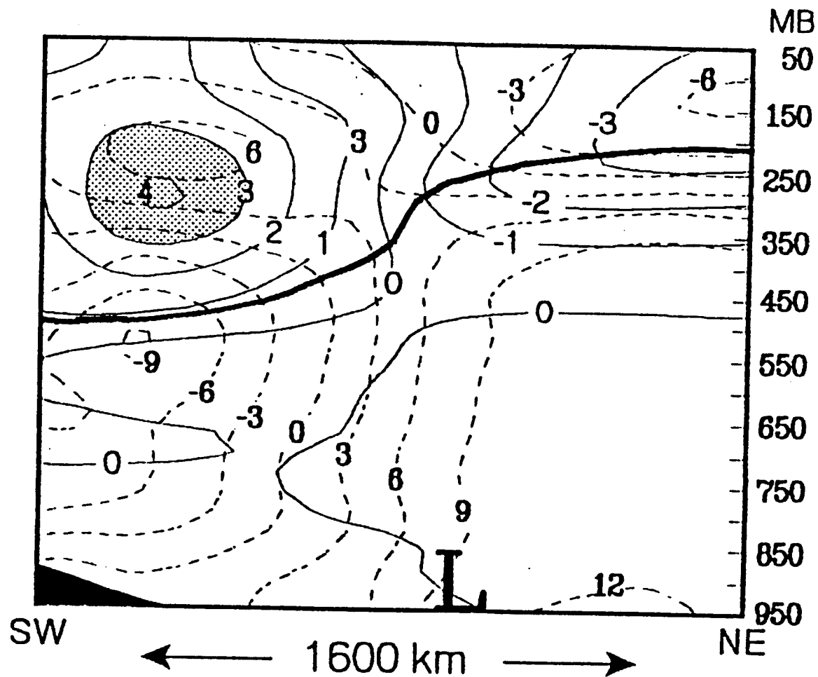
Figure 2. Southwest to northeast cross section of observed perturbation isentropic PV (solid, 10^{-4} \text{ m}^2 \text{ s}^{-1} \text{ K kg}^{-1} ) and perturbation temperature (dashed, K). Stippling denotes regions with anomalously high values of PV. The dynamic tropopause (PV value of [1.0 \times 10^{-4} \text{ m}^2 \text{ s}^{-1} \text{ K kg}^{-1}] ) is denoted by a heavy solid line and the position of the surface low by an "L". From Hirschberg and Fritsch (1991a).
