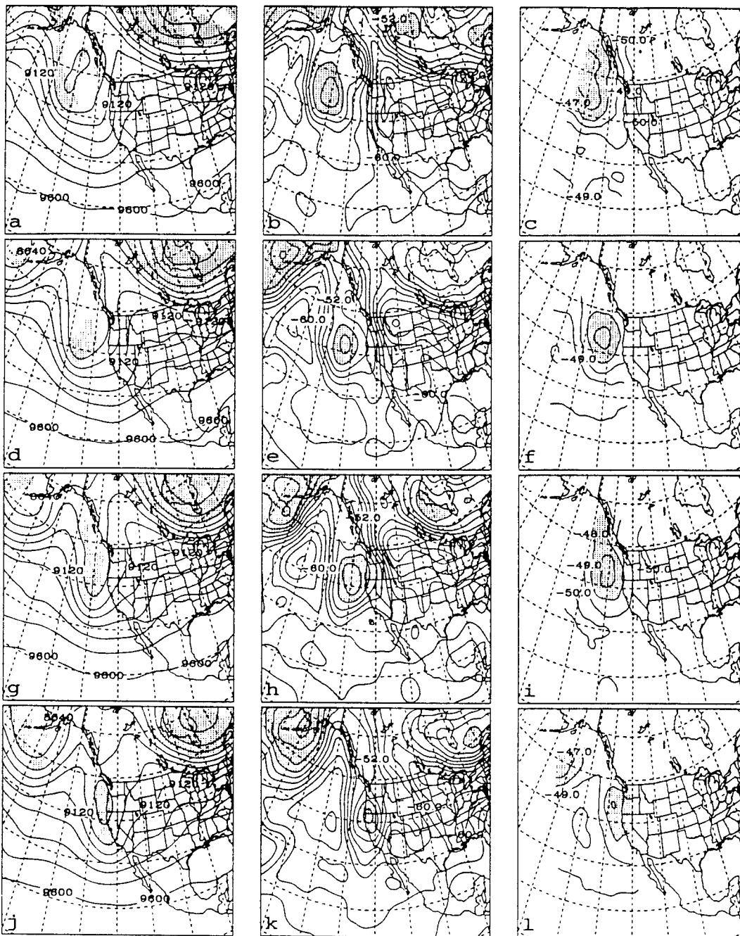
Figure 22. Horizontal analyses of 300-mb height (solid, contour interval 120 m) and PV (values > 5.0 PV units dot filled)[a,d,g,j]; 200-mb temperature (contour interval 2°C)[b,e,h,k]; and channel 3 MSU brightness temperature (contour interval 1°C)[c,f,i,l] for 23/1200, 24/0000, 24/1200, and 25/0000, respectively. Lower left latitude-longitude value is 10° N, 150° W. Latitude-longitude increment is 10°.
