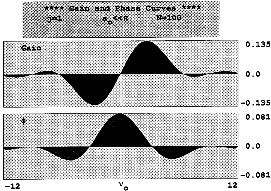
Figure 6 - Weak fields, low current anti-symmetric gain spectrum
