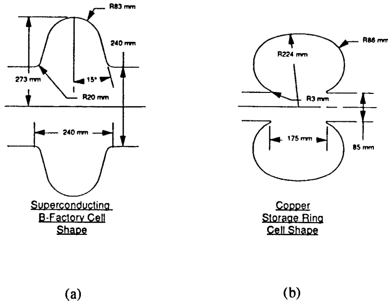
Figure 11 - Typical accelerator cells, (a) superconducting (b) room temperature. From Ref. [15]
