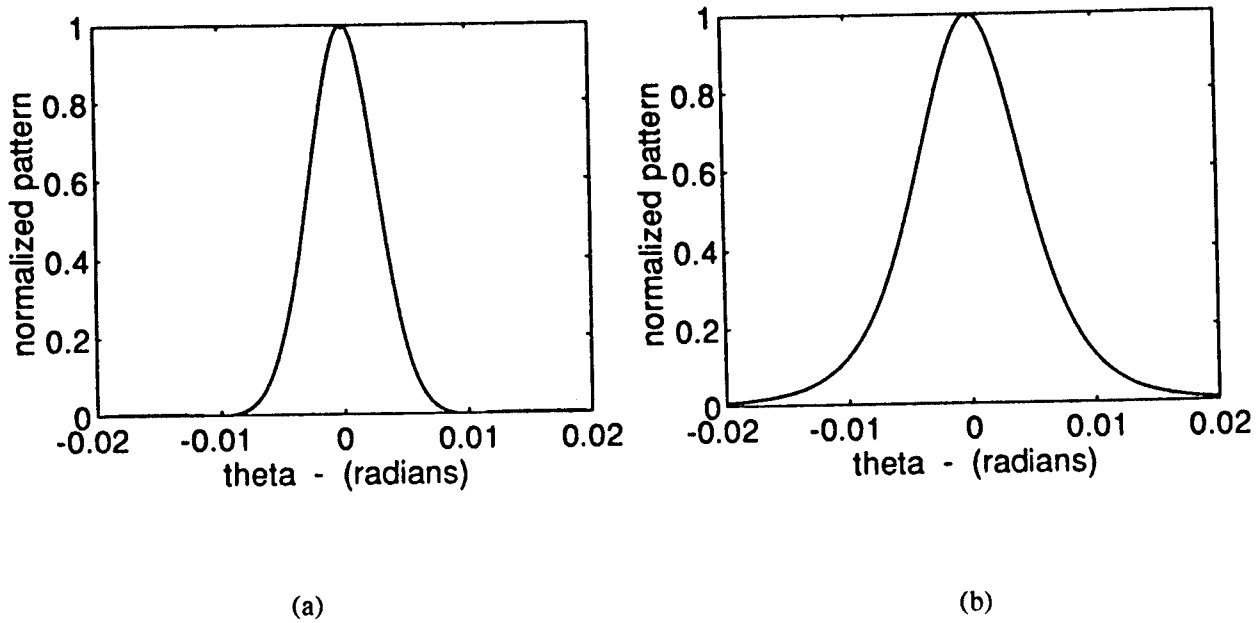
Figure 3 - Radiation pattern from a relativistic electron ( \gamma = 100 ) under a transverse acceleration, (a) \phi = 0 , (b) \phi = \pi/2
