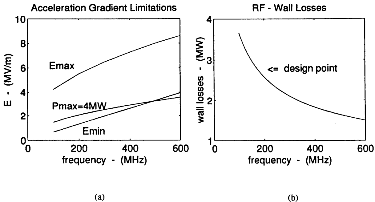
Figure 13 - RT accelerator (a) field strength requirements, and (b) wall losses
