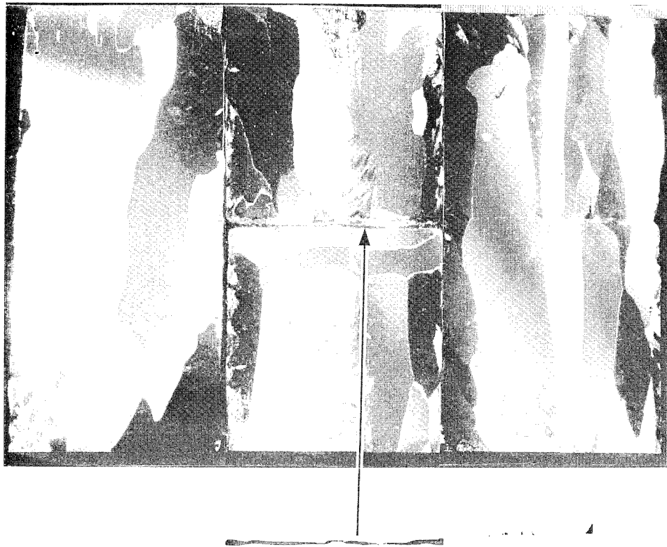
Figure 8. Thin sections showing the effect of no. 2 fuel oil on the growth of freshwater ice.
