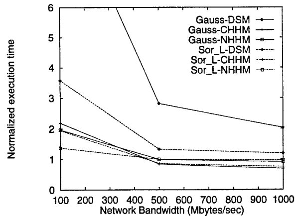
Figure 11: Normalized execution time for DSM and Cashmere protocols under different network bandwidths (64 processors).
