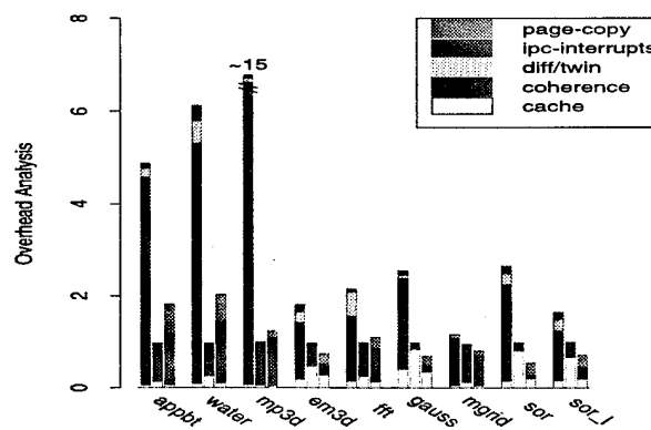
Figure 3: Overhead analysis for DSM and Cashmere protocols on 64 processors.
