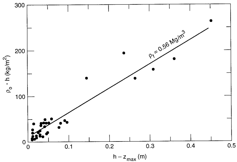
Figure 6. Vehicle sinkage analysis. (From Richmond et al. 1990.)
