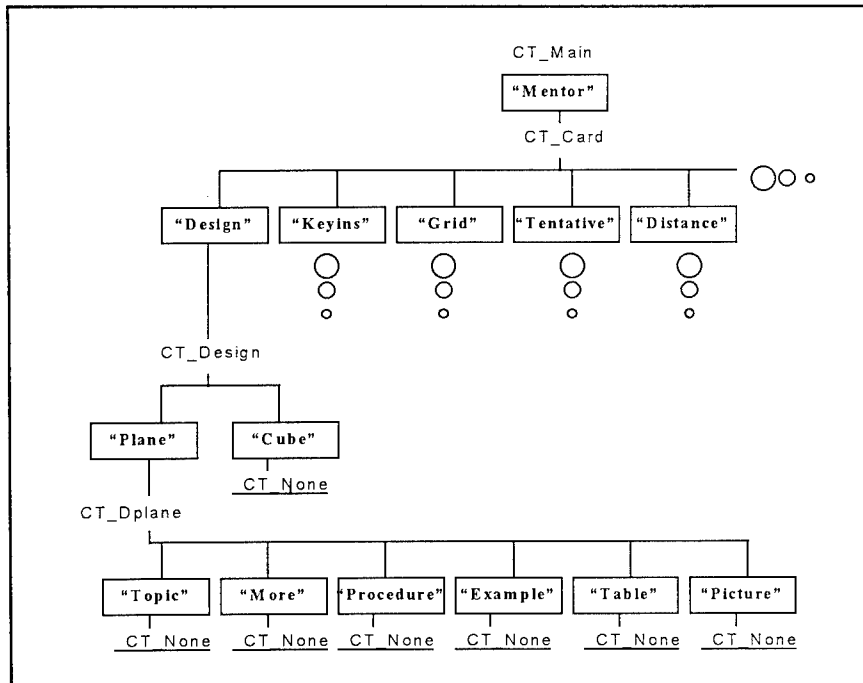
Figure 26. Organization of a command table.
