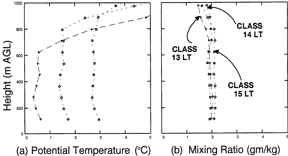
Figure 11. CLASS potential temperature (a) and water vapor mixing ratio (b) profiles observed at 13, 14 and 15 LT 12 March 1992.
