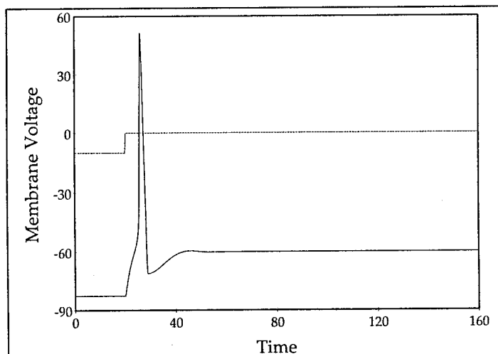
Figure 2. A -10 \mu\text{A} current pulse is used to hyperpolarize the cell membrane to -80 \text{ mV} for a very long time. After release from hyperpolarization at 20ms, a single action potential occurs, without any stimulation. The current causing hyperpolarization is shown with dashed line and membrane potential is shown in solid line.
