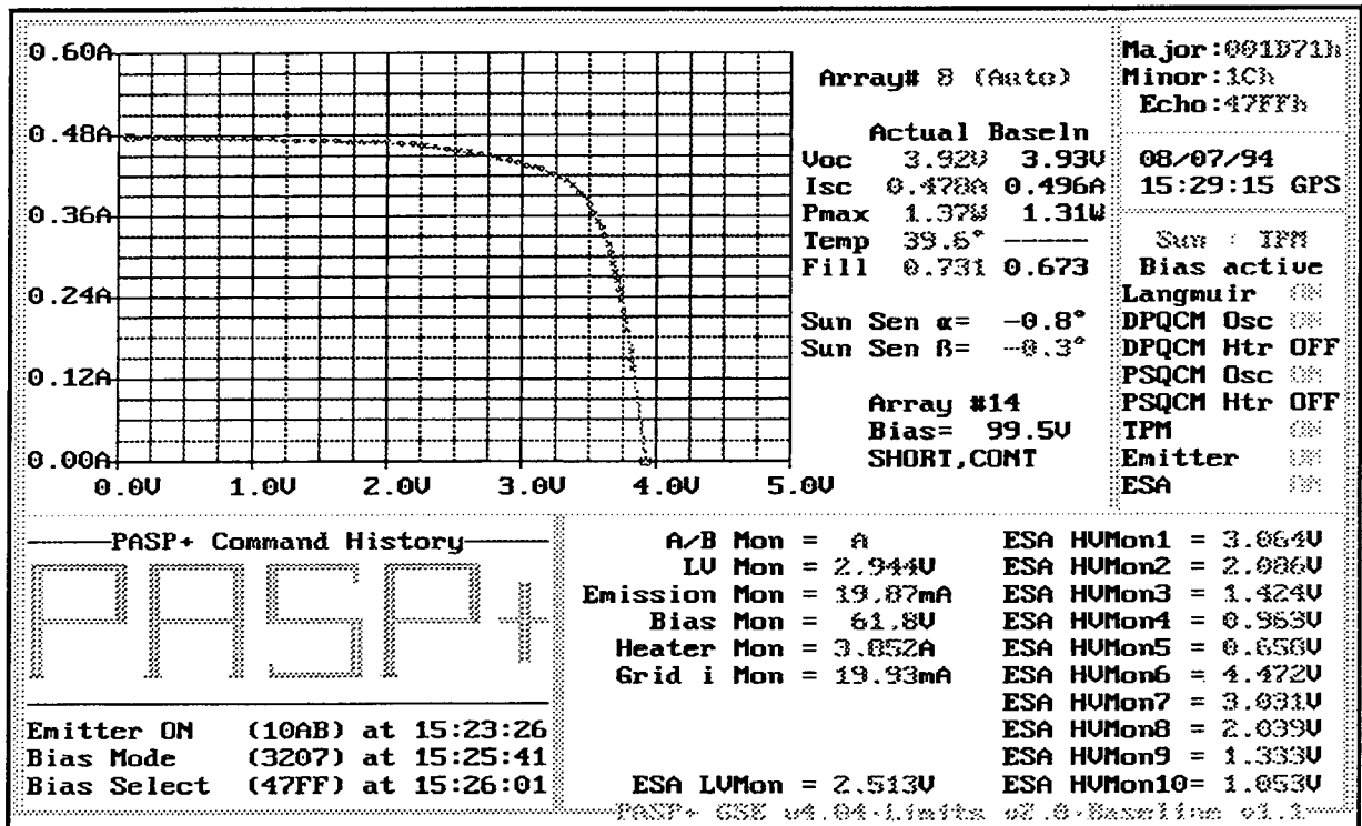
FIGURE 8: REAL-TIME EMITTER & ESA MONITOR VOLTAGE DISPLAYS
