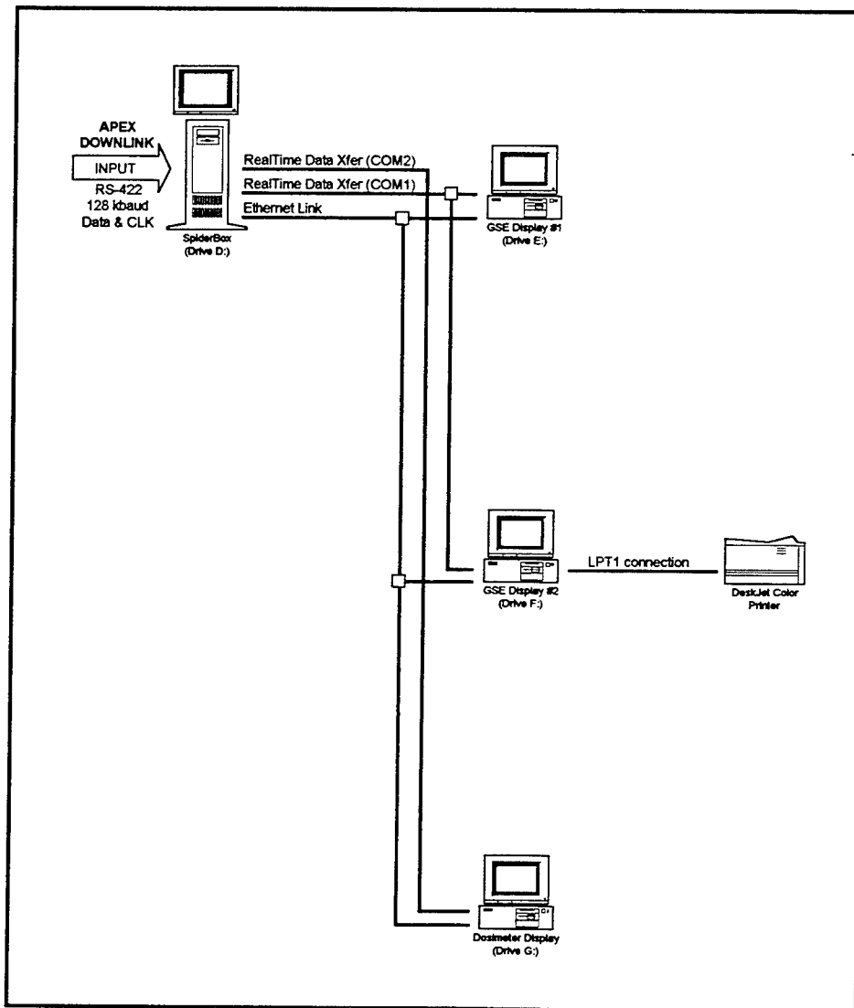
FIGURE 1: PASP PLUS GSE DATA DISPLAY NETWORK
