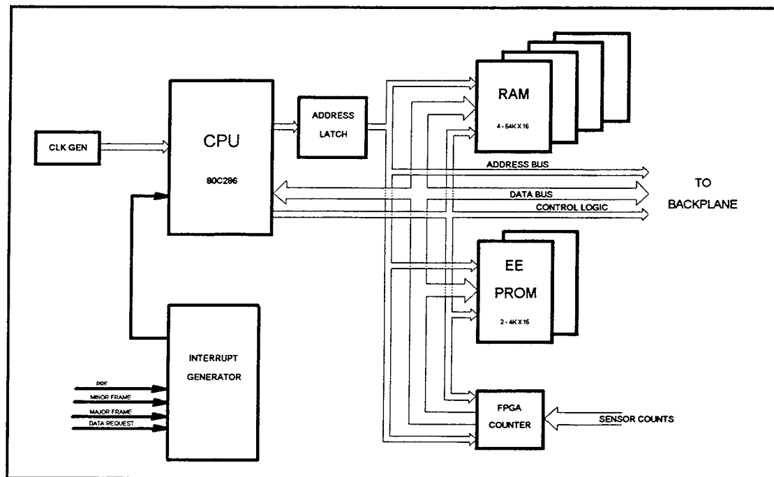
FIGURE 20: CENTRAL PROCESSOR BOARD SCHEMATIC
