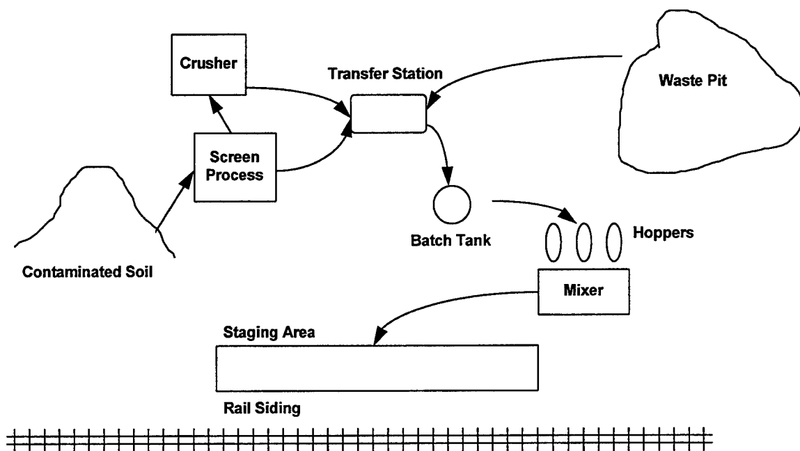
Figure 3.4. Cementation Plant
