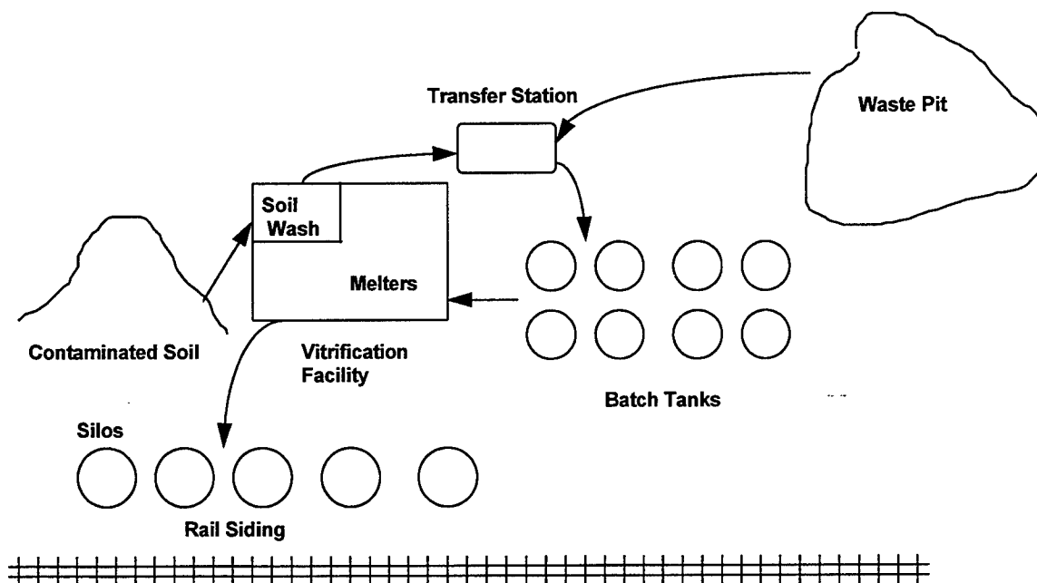
Figure 3.3. Vitrification Plant
