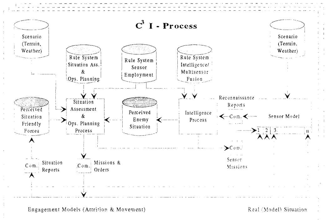
Figure 2.5: Basis Structure of the C³I-Process
