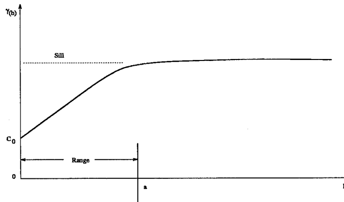
Figure 2.7 Spherical Model
