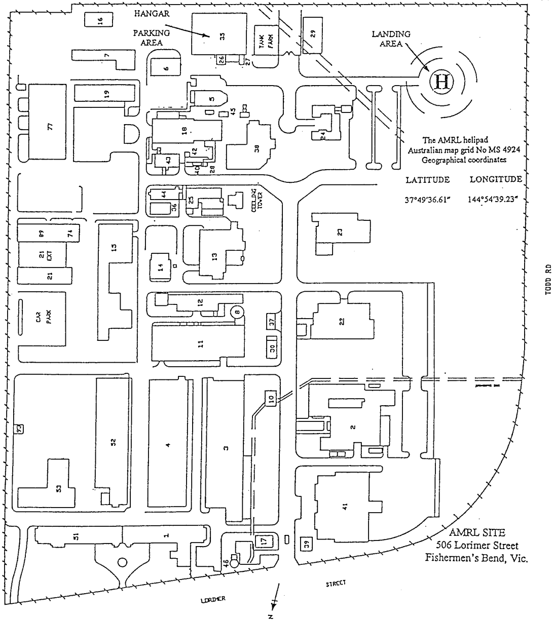
Figure 5: AMRL Site Plan showing aircraft landing and parking locations
