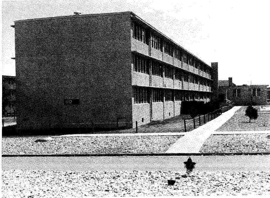
Figure 1. Building 812: Type 64 (L-shaped) Barracks With EIFS Installed.
