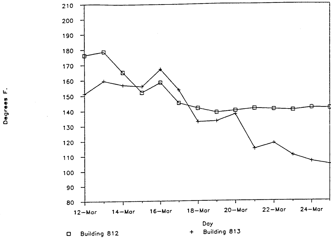
Figure 17. Hot Water Supply Temperature: Zone 2.
