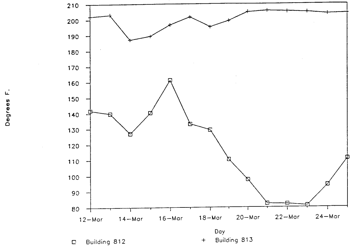
Figure 18. Hot Water Supply Temperature: Zone 3.
