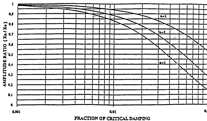
Figure 7: Amplitude ratio vs. Fraction of critical damping.
