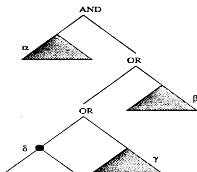
Figure 5: A small change in a Boolean tree will not necessarily determine a sharp change in the program behavior.
