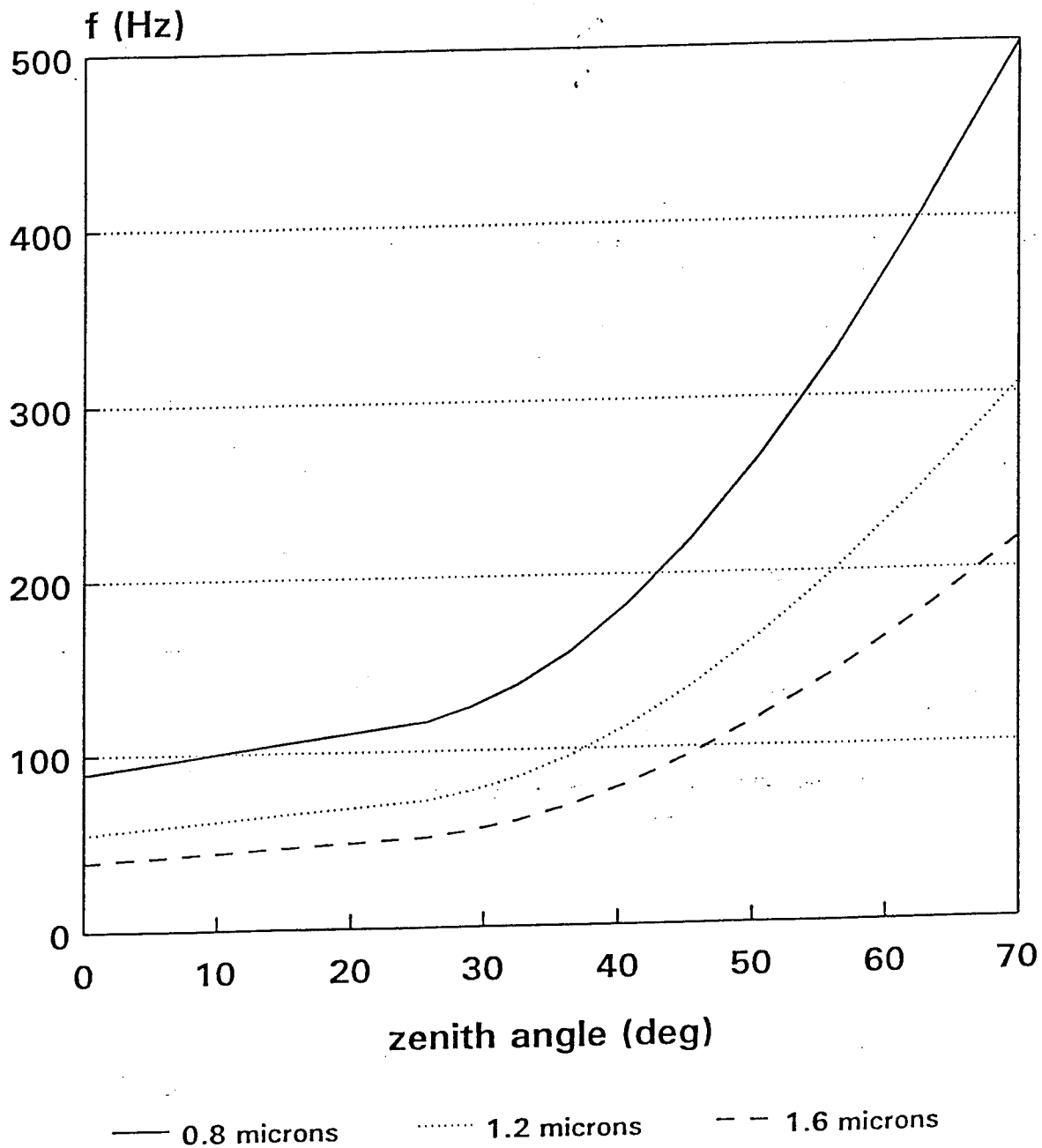
Figure 9: Greenwood frequency f_G vs. zenith angle for Beland night turbulence model at \lambda = 0.8, 1.2, \text{ and } 1.6 \mu m .
