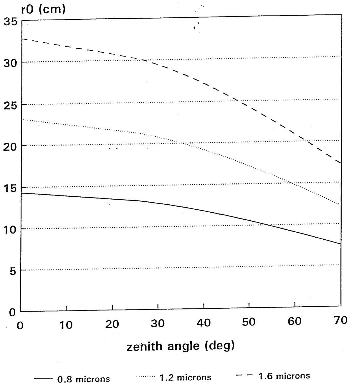
Figure 8: Fried coherence diameter r_0 vs. zenith angle for Beland night turbulence model at \lambda = 0.8, 1.2, \text{ and } 1.6 \mu\text{m} .
