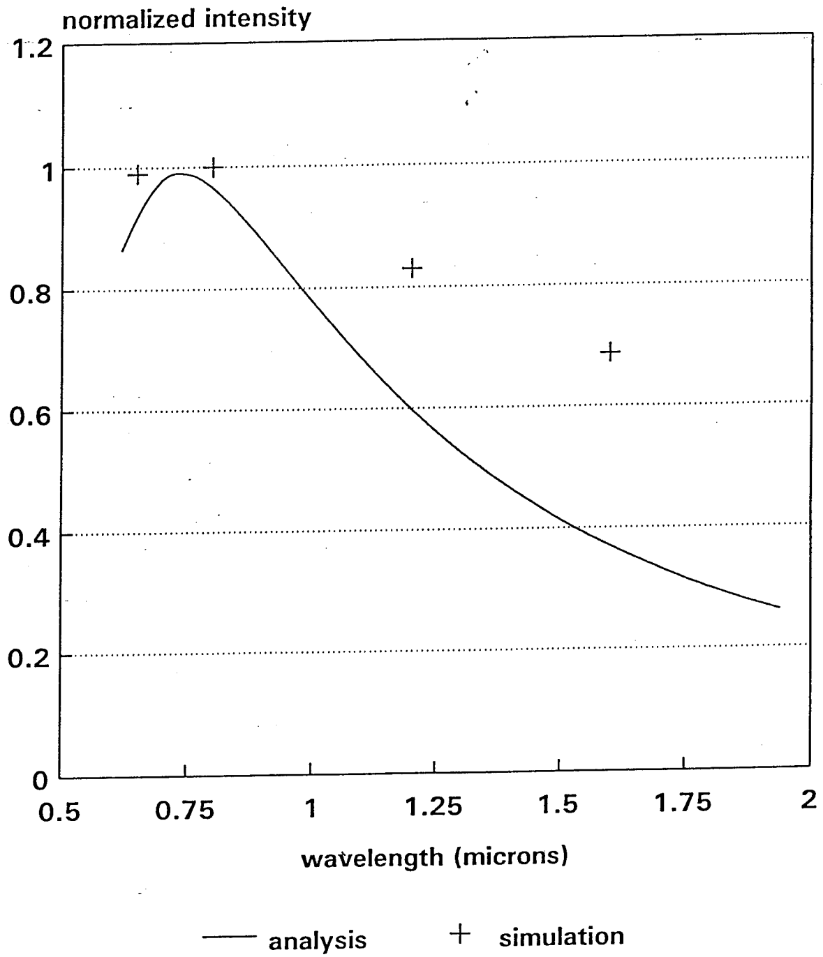
Figure 3: Correspondence between simulation I_n vs. \lambda and predicted on-axis intensity curve for a 741-actuator system with r_o = 18 cm at \lambda = 0.8 \mu\text{m} .
