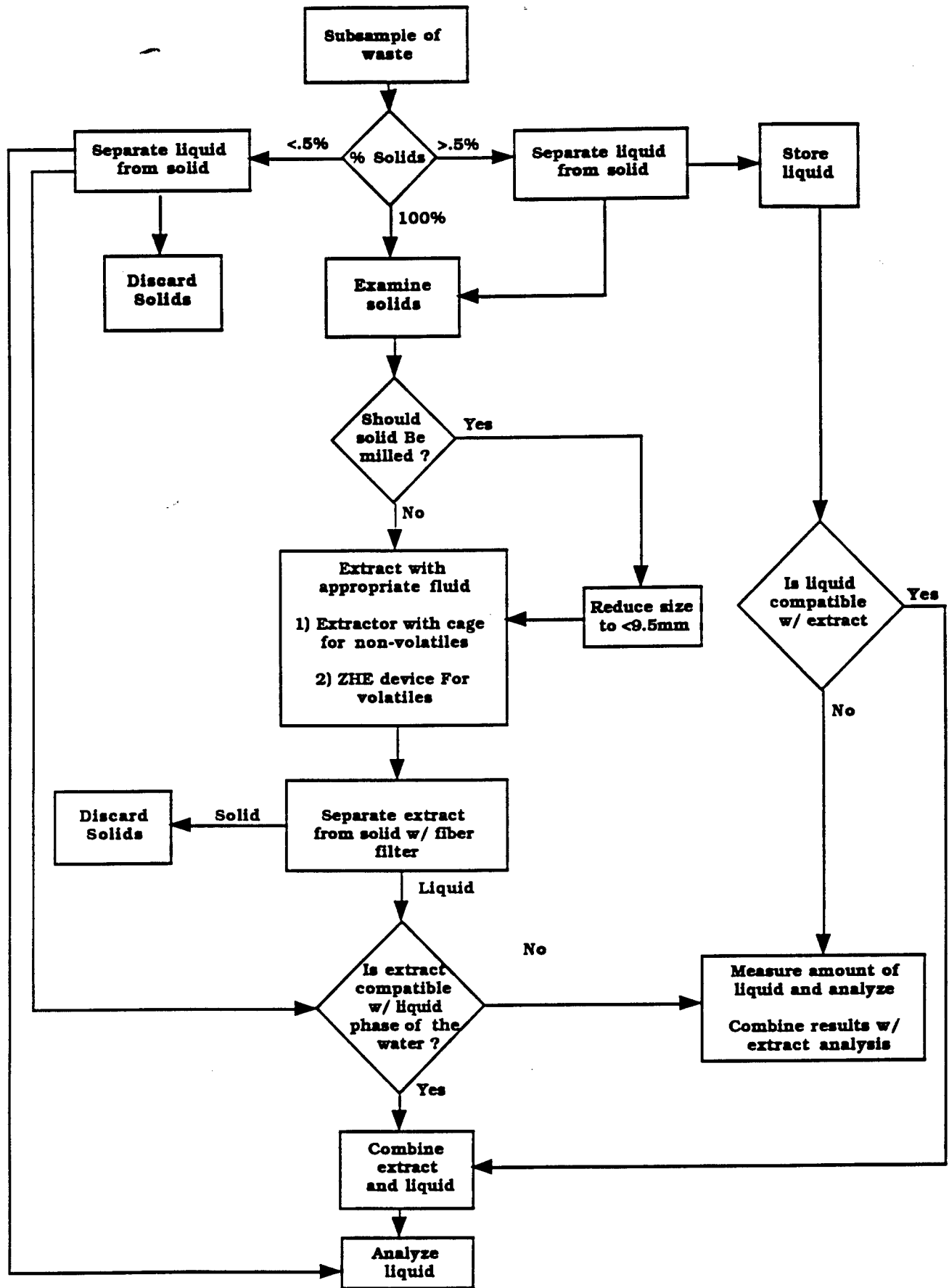
Figure 2. TCLP Procedure.
