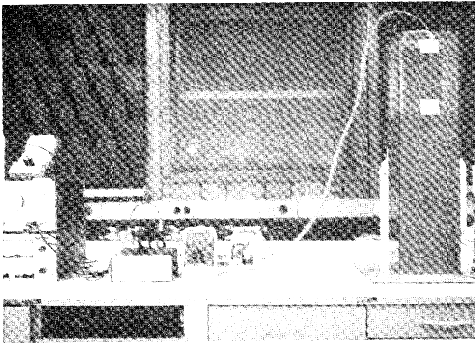
Figure 30. Laboratory scale resistivity probe
