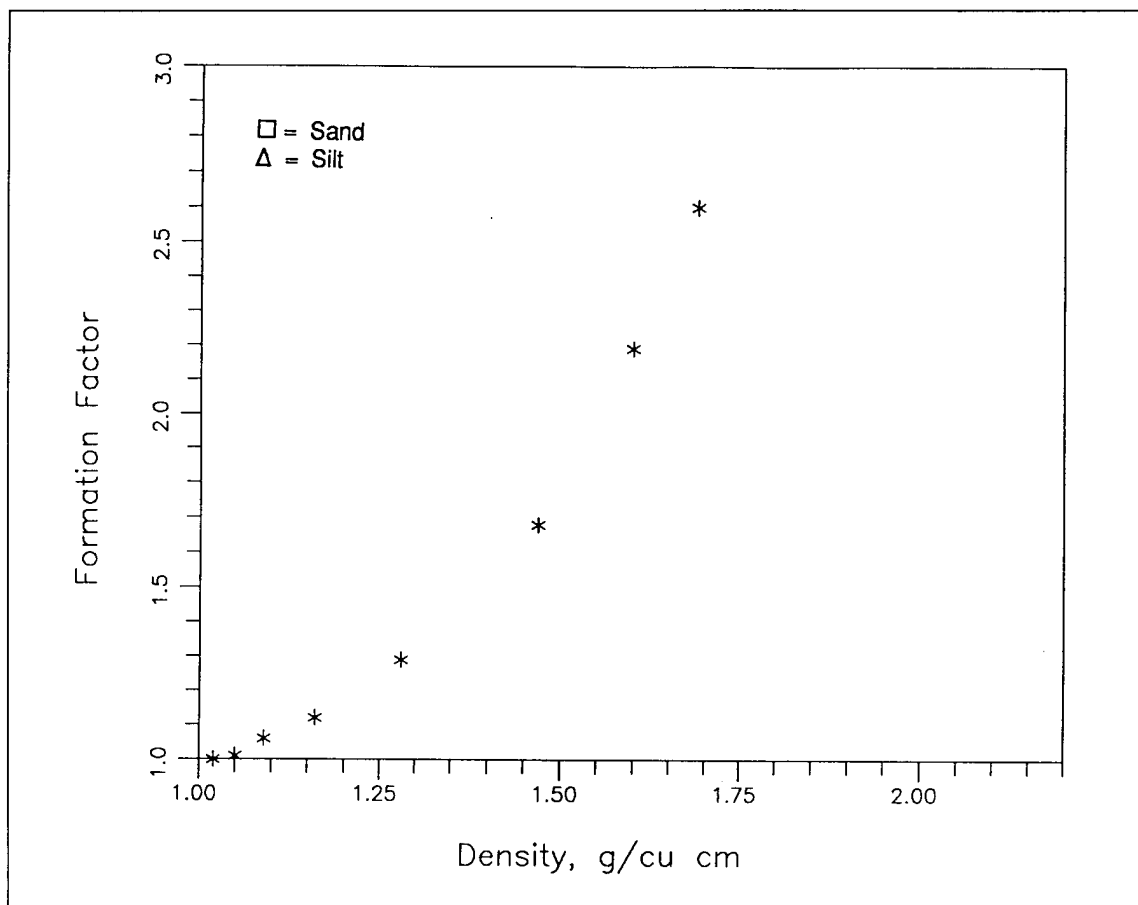
Figure 32. Resistivity calibration curve for a sand, silt, and clay mixture
