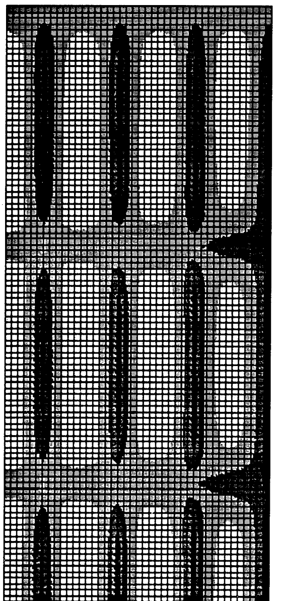
FIGURE 4.8 HSS PLATE MODEL 2; \sigma_{yy} STRESS (VIEW FROM THE BOTTOM)
