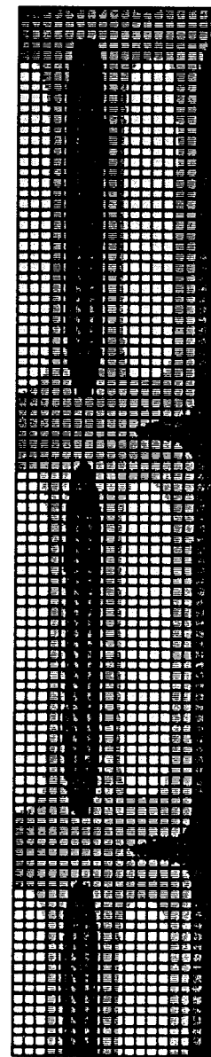
FIGURE 4.10 OSS PLATE MODEL 3; \sigma_{yy} STRESS (VIEW FROM THE BOTTOM)
