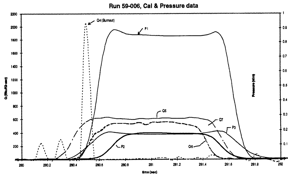
Figure 24. Typical Calorimeter and Pressure Response Data
