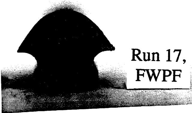
c) Profile, Fore
