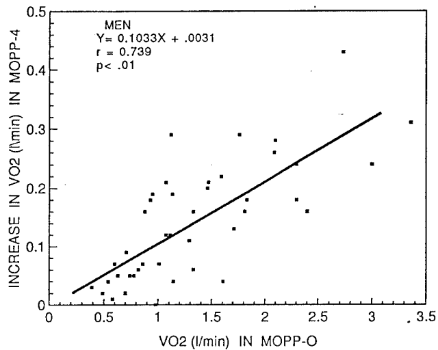
Figure 3. Relationship between energy cost in MOPP 0 and the absolute ( l \cdot min^{-1} ) increase in Vo_2 with MOPP 4.
