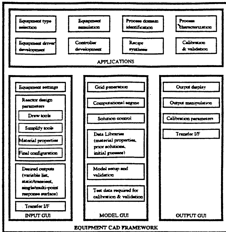
Fig. 5: Suggested equipment CAD framework for process synthesis.
