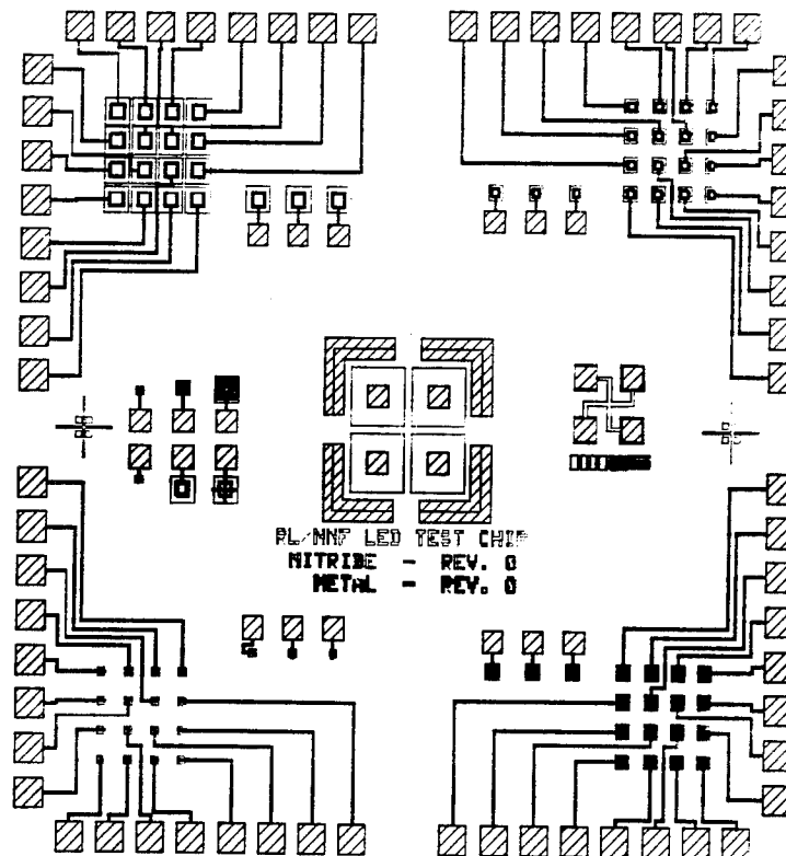
Figure 7. CAD layout of LED chip.
