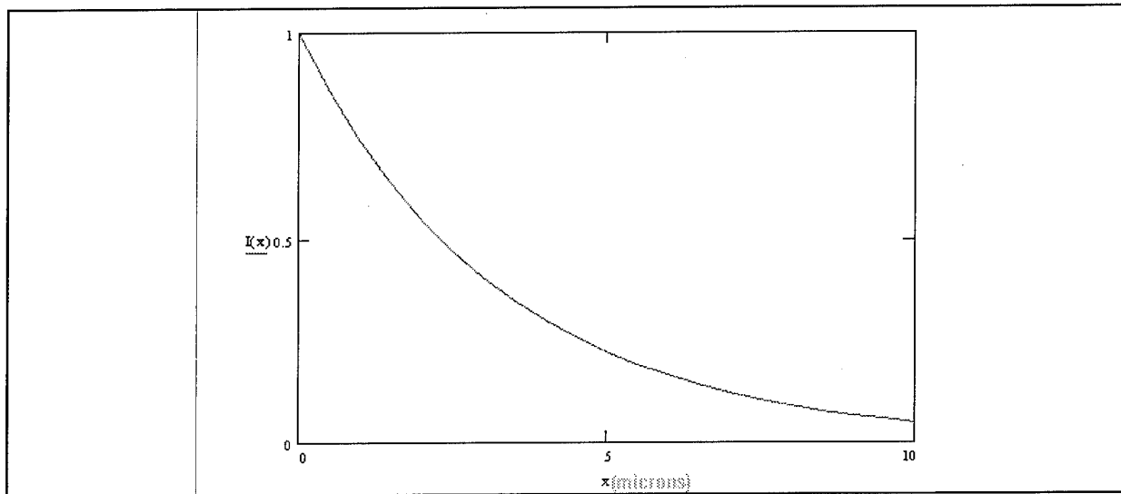
Figure 12. Intensity at a depth x of an arbitrary intensity of "1" just under Si surface for 655nm light.
