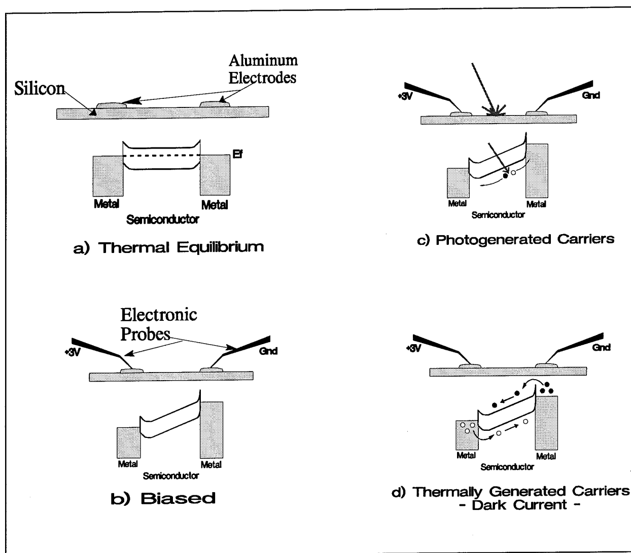
Figure 13. The energy diagram of metal-semiconductor-metal photodetectors under 4 operating modes: a) unbiased, no illumination, b) biased with no illumination, c) biased and illuminated, and d) biased with no illumination.
