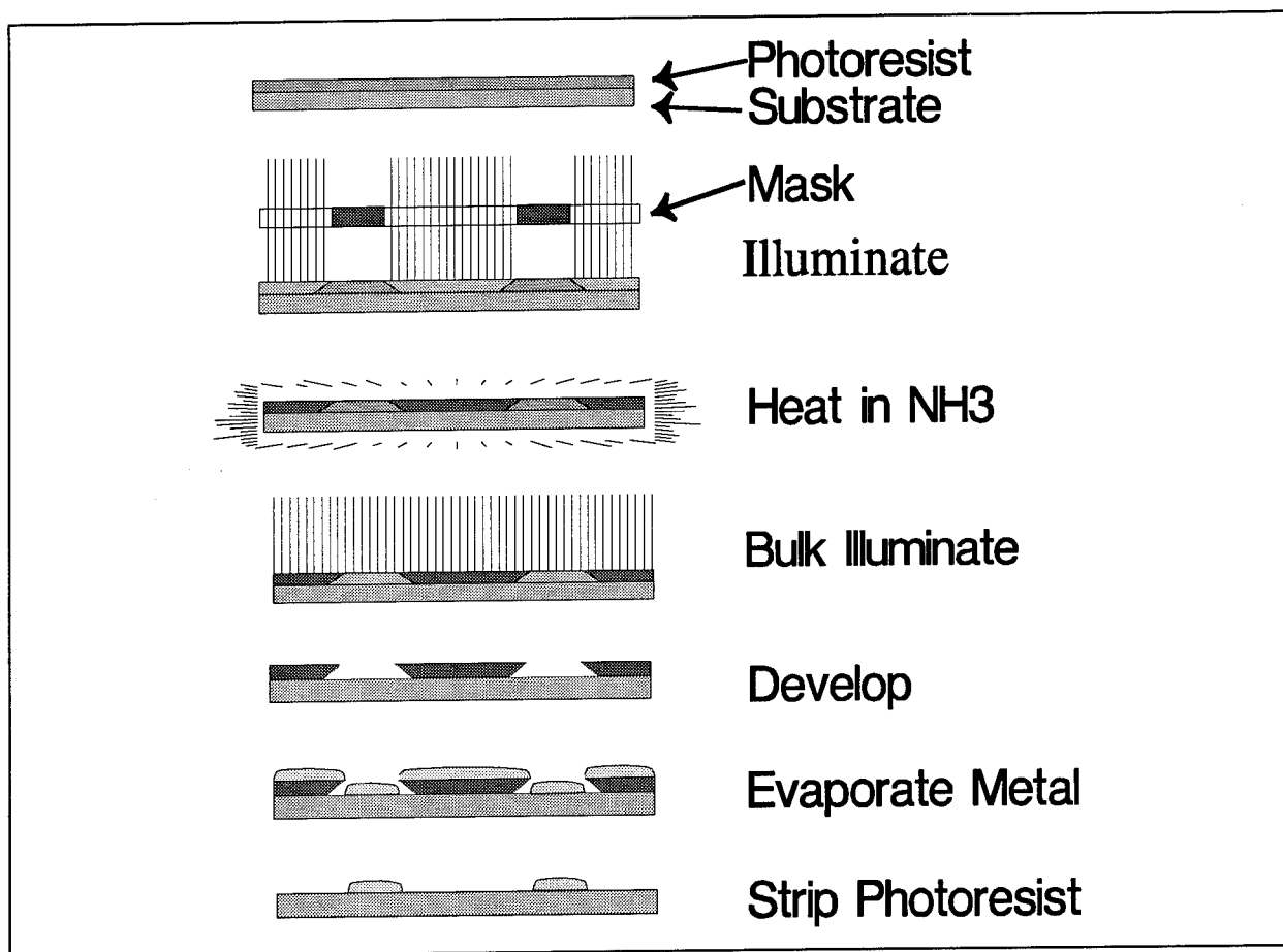
Figure 14. The "lift-off" procedure for depositing metal electrodes on a substrate.
