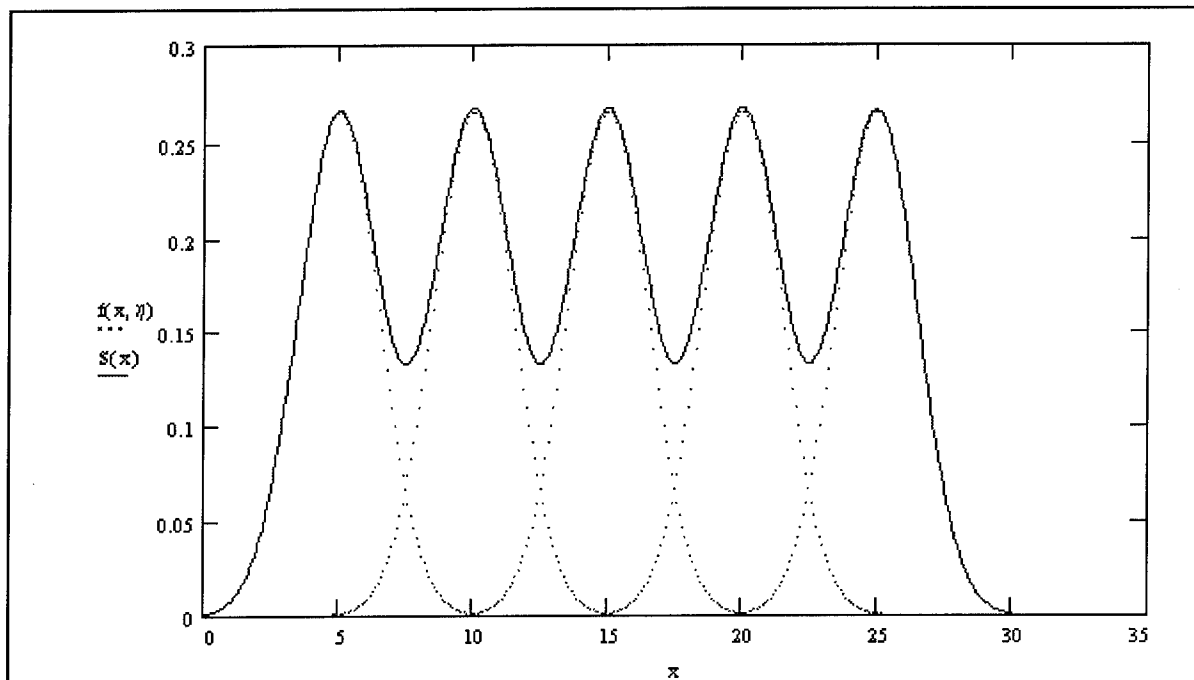
Figure 5. Overlapping e-beam gaussian exposures. The solid line represents the net exposure recorded in the e-beam resist.
