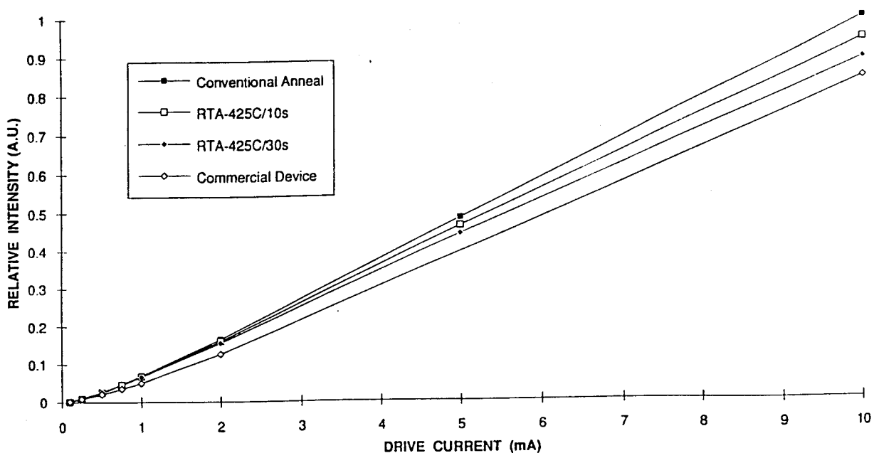
Figure 8. Relative intensity-current measurements for LED's fabricated with conventional two-step furnace anneal cycle, and two single rapid thermal anneal cycles: 425°C/10s and 425°C/30s, as well as commercially available devices.
