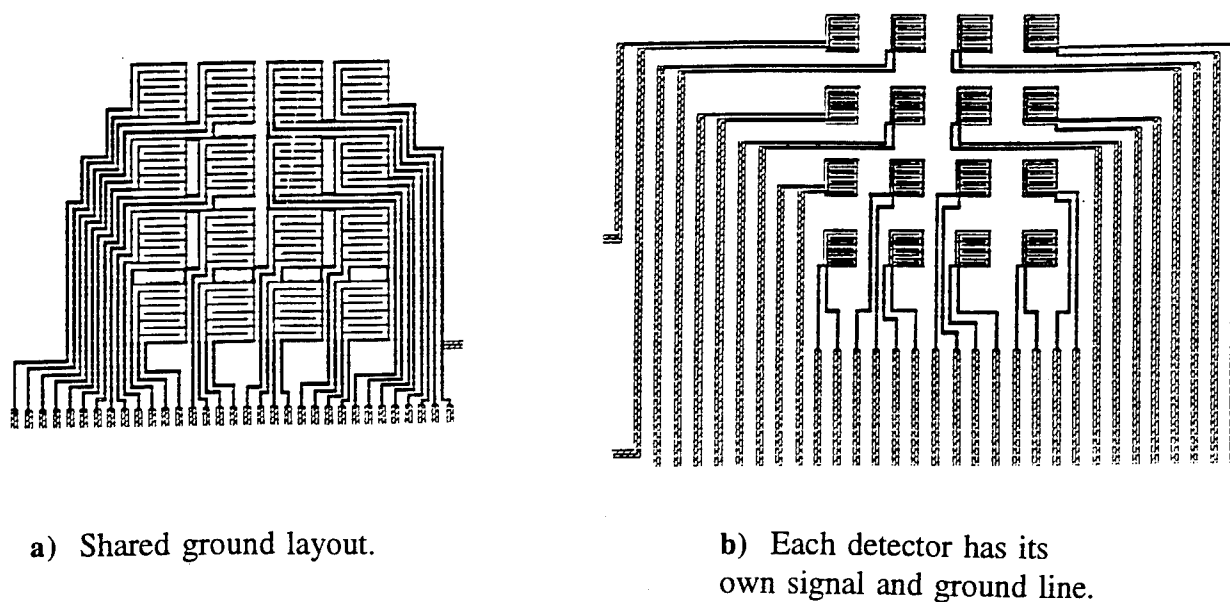
Figure 11. Metal-semiconductor-metal photodetectors in 2 array configurations.
