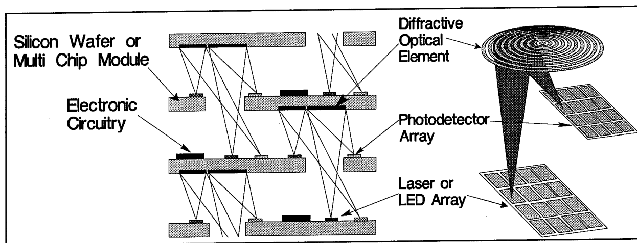
Figure 1. A plane-to-plane 16 channel optical interconnect using a diffractive optic element (DOE) to focus and redirect the light from an array of light emitting diodes (LEDs) to an array of photodetectors.
