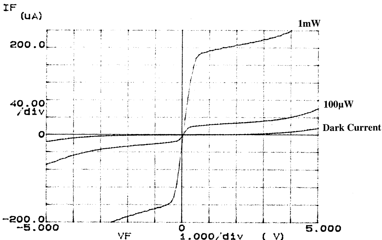
Figure 15. I/V curves of an MSM photodetector with Al metalization on an n-type Si wafer. The bottom curve shows the device dark current. The middle and top curves show the induced photocurrent with 100 \mu W and 1mW of 780 \mu m light incident on the detector.
