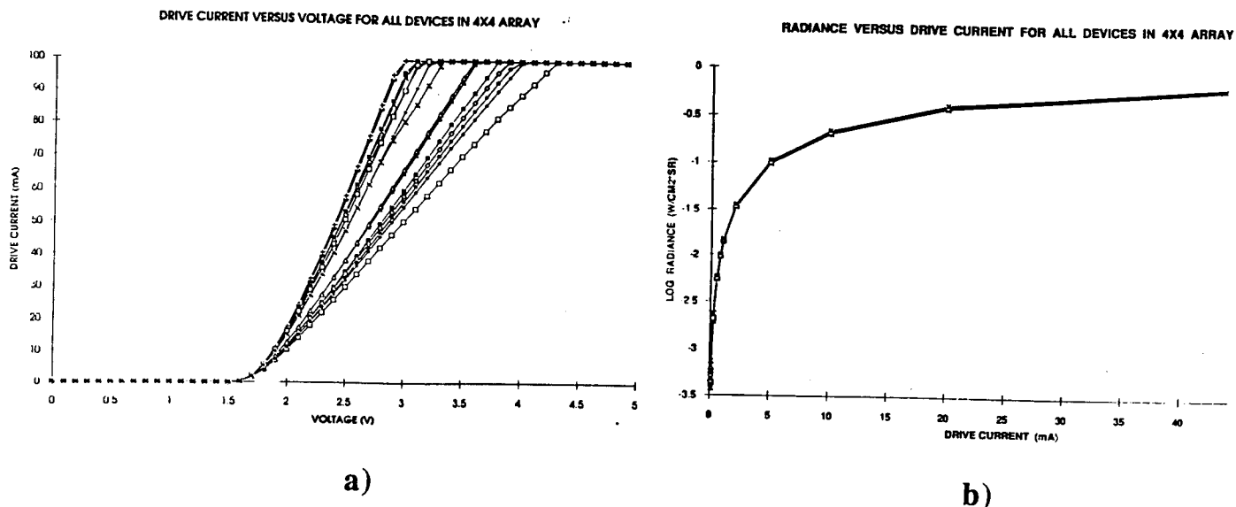
Figure 9. Uniformity of GaAsP LED's (junction area 50 X 50 \mu m) in a 4X4 array - each symbol represents a separate device in the array: a) current-voltage measurements with 100mA compliance limit and b) radiance-current measurements.
