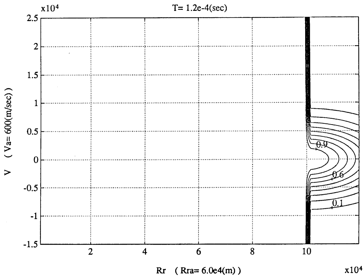
Fig. 4-11: Bistatic ambiguity function for the Gaussian pulse for the case considered
