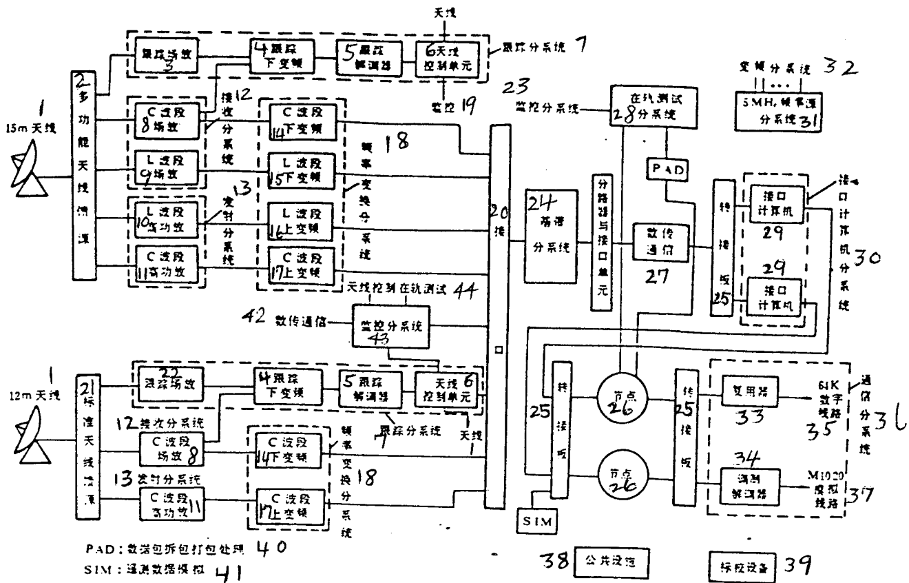
Fig. 4. Block Diagram for Beijing TT&C Station KEY: 1 - Antenna 2 - Multifunctional antenna feed source 3 - Transmission by tracking field 4 - Down conversion of tracking 5 - Tracking demodulator 6 - Antenna control element 7 - Tracking subsystem 8 - Field transmission of C-band 9 - Field transmission of L-band 10 - High-power transmission of L-band 11 - High-power transmission of C-band 12 - Receiving subsystem 13 - Transmission sub- system 14 - Down-conversion of C-band 15 - Down-conver- sion of L-band 16 - Up-conversion of L-band 17 - Up conversion of C-band 18 - Frequency-transfer subsystem 19 - Monitoring and control 20 - Interface 21 - Standard antenna feed source 22 - Transmission of tracking field 23 - Monitoring and control subsystem 24 - Base band transmission 25 - Switchboard 26 - Nodal point 27 - Data transmission communication 28 - In-orbit test subsystem 29 - Interface computer 30 - Interface computer subsystem 31 - Frequency source subsystem 32 - Variable frequency subsystem 33 - Repeater 34 - Modem 35 - 64K digital circuits 36 - Communication subsystem 37 - Analog circuits 38 - Common-use utilities 39 - Marking and calibration equipment 40 - Unpacking and packing of data packet 41 - Remote-sensing data simulation 42 - Data communication 43 - Monitoring and control subsystem 44 - Antenna control in-orbit testing
