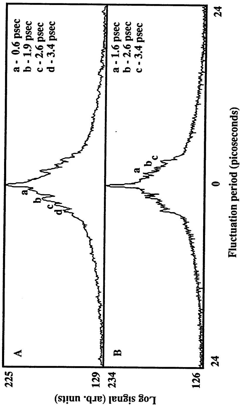
FIG. 4 Fourier transform of backscattered frequency spectrum: A) hydrogen, B) helium.
