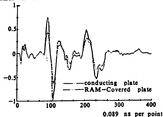
Fig.7 Scattering Echoes Associated with Plates
