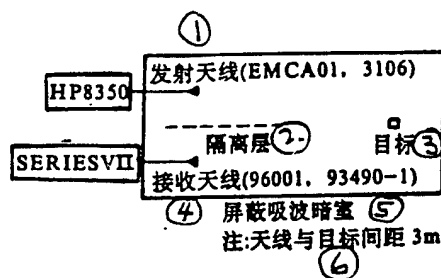
Fig.1 Frequency Domain Test Measurement Block Diagram
