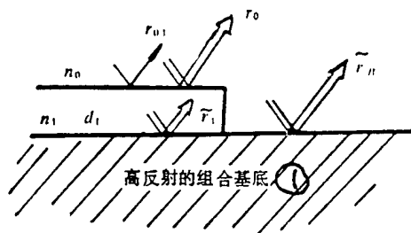
Fig.1 Symbol Conventions
