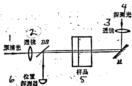
Fig.1 Photothermal Deflection Technique Schematic
