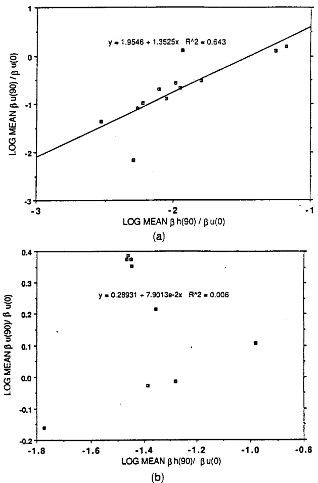
Fig. 3. Same measurements as shown in Fig. 2 but normalized to the unpolarized forward scattering, \beta_u(0) , for (a) algae and (b) microspheres. Normalization is mean \beta_u(90) divided by mean \beta_u(0) .
