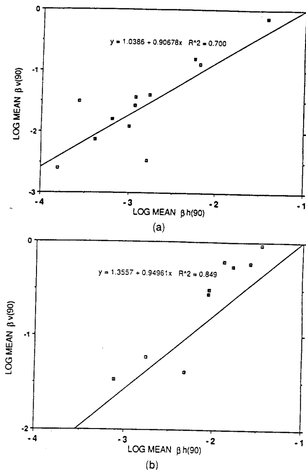
Fig. 4. Log of the mean value of the copolarized light scattering measured at 90^\circ , \beta_v(90) , versus the log of the mean value of the cross-polarized light scattering measured at 90^\circ , \beta_h(90) , for (a) algae and (b) microspheres.
