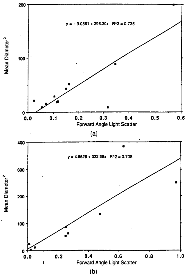
Fig. 1. Mean values of the forward-angle light scattering as measured on the flow cytometer for varying cross sections (given as the square of the equivalent spherical diameter) of (a) algae and (b) microspheres.
