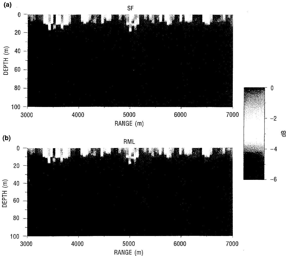
Fig. 9—Comparison of SF in the “large” sector limit and RML. Ambiguity surfaces are calculated for a source placed at 5000-m range and 15-m depth in the waveguide, with -40\% mismatch of the sound speed profile. A 700\text{-m} \times 40\text{-m} sector was used for the SF case. The surfaces are indistinguishable. (a) SF, PBR = 9.27 dB and (b) RML, PBR = 9.27 dB.
