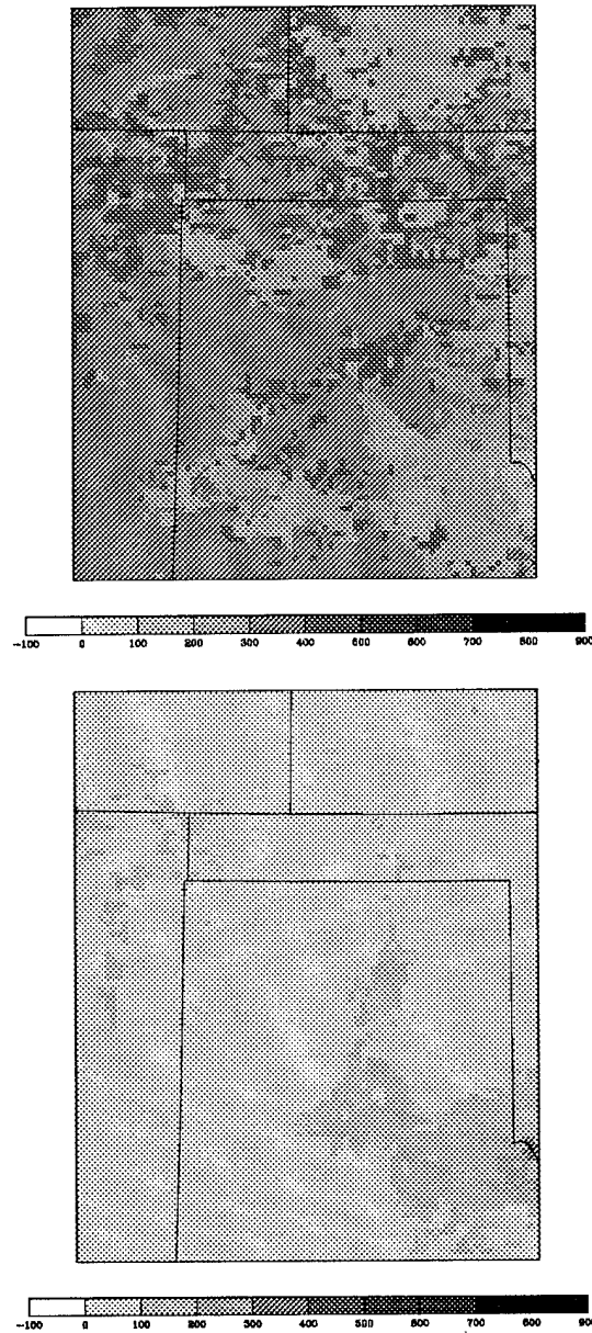
Figure 3.2: Sensible heat flux (top) and latent heat flux (bottom) at 2000 UTC from the 50SM simulation. Values are in W m^{-2} .
