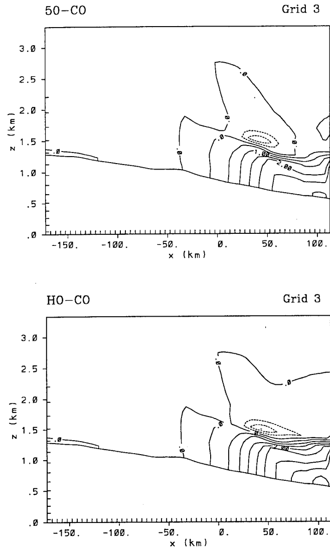
Figure 4.4: 50SM minus CONT (top) and H0MD minus CONT (bottom) virtual potential temperature difference (K) at 1800 UTC for same cross section as 4.1. Contour interval of 0.5 K.
