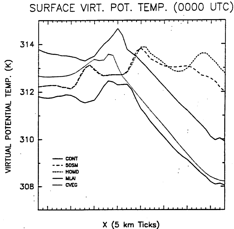
Figure 4.7: Same as 4.6 for virtual potential temperature (K).
