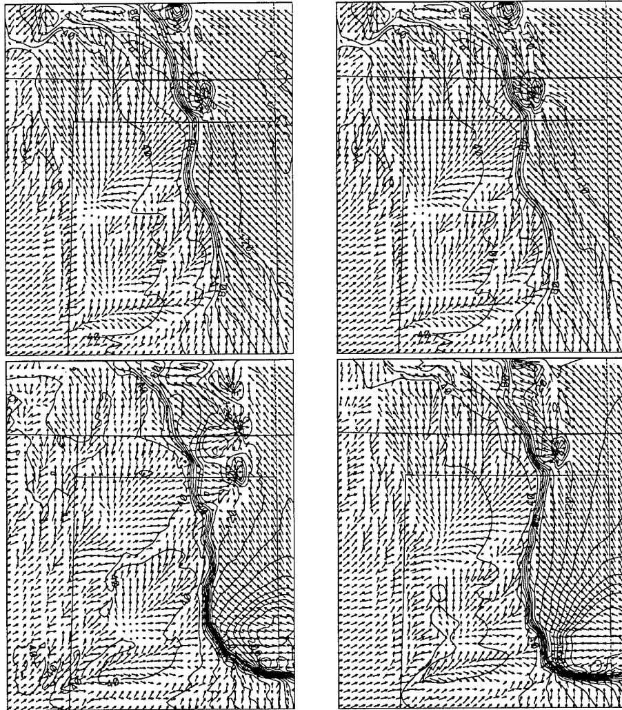
Figure 4.16: Same as 4.15, but for the 50SM run (top-left), HOMD run (top-right), MLAI run (bottom-left), and CVEG run (bottom-right).
