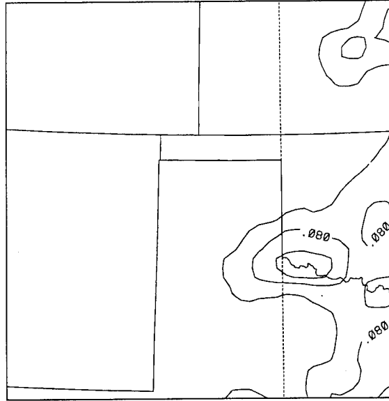
Figure 3.1: Volumetric soil moisture analysis 50SM simulation on grid 2. Contour interval is 0.04.
