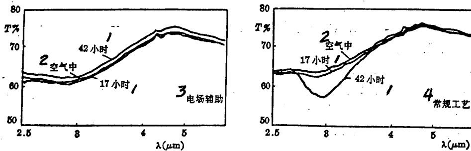
Fig. 6. Measured transmission property of \text{Air} | (\text{HL})^2 \text{H}4\text{LH}(\text{LH})^2 | \text{Al}_2\text{O}_3 ( \lambda_0 = 560\text{nm} ) in 3micrometer water absorption band KEY:1 - hours 2 - in air 3 - electric field-assisted 4 - conventional technique
