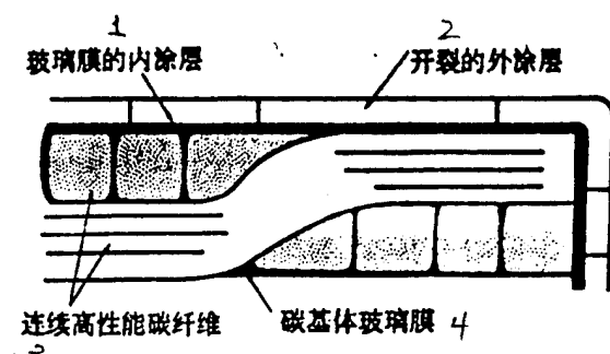
Fig.3 C/C Composite Material Oxidation Protection System
