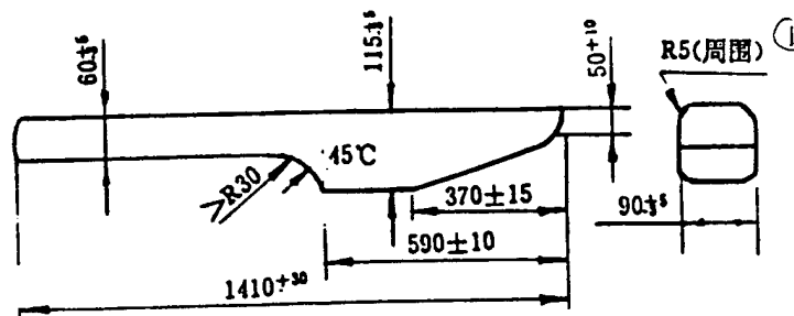
Fig.2 Lower Cabin Connector Premanufacture Stock Diagram (1) Peripheral Contour
